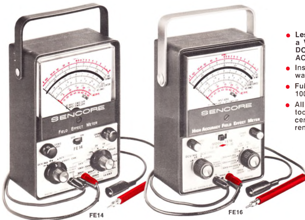
Special shielded input leads prevent RF pickup.
