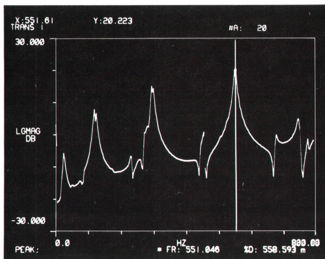
Fig. 8. A result of the measurement of Fig. 7 for one point on the plate surface. The resonance at 551 Hz (identified by the X cursor) represents a mode of vibration with a damping factor of 0.559%.
