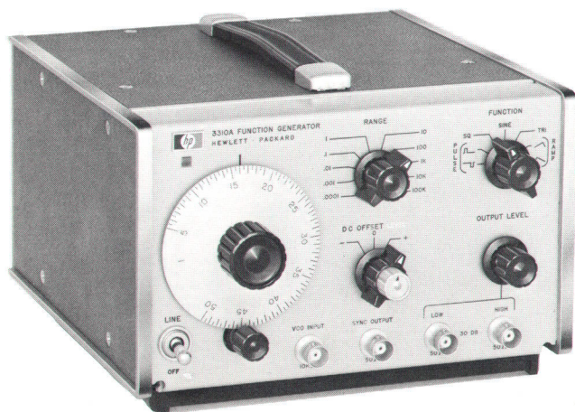
Fig. 1. This new HP Model 3310A Function Generator has a frequency range from 0.0005 Hz to 5 MHz and generates sine, square, and triangular waves as well as pulses and ramps.
