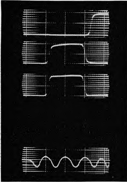
Figure 12. Oscillogram illustrating testing of delay line or delay cable
