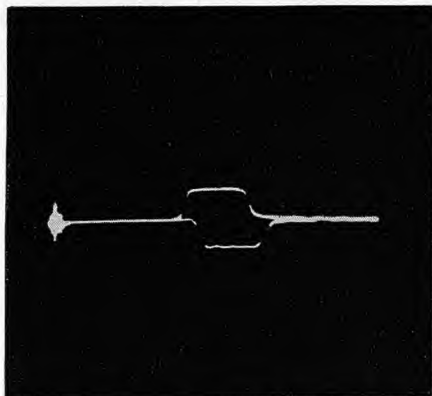
Figure 35. Oscillograms of improperly adjusted grid and plate delays
