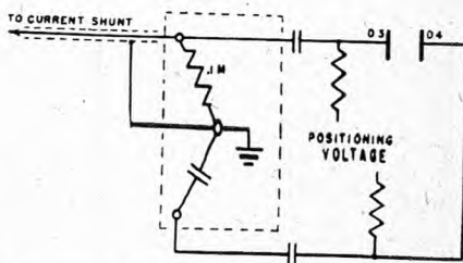
Figure 22. Long deflection plate ground return circuit
