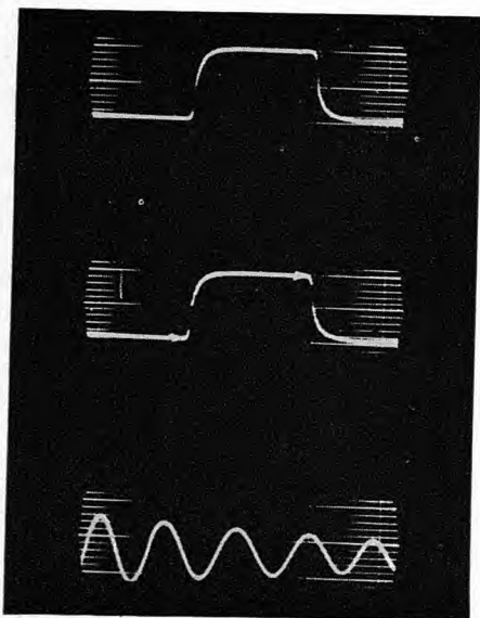
Figure 21. Effect of ground loop difficulty in connection with use of delay line
