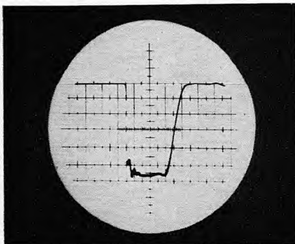
Figure 26. Pulse forming network oscilloscope, resulting from incorrect measuring techniques
