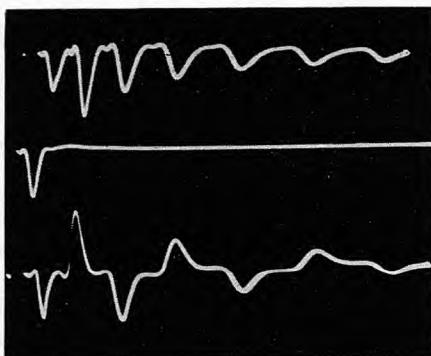
Figure 10. Oscillogram of line impedance measurements made with pulses
