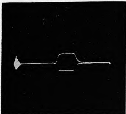
Figure 34. Oscillograms of properly adjusted grid and plate delays superimposed
