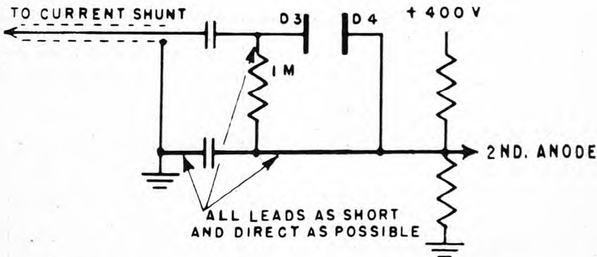
Figure 24. Reduced deflection plate ground return circuit
