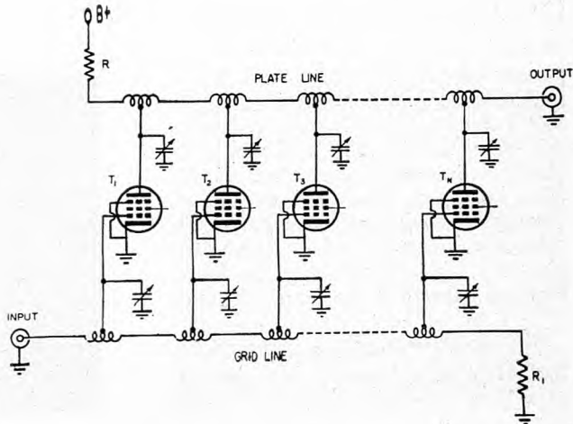
Figure 33. Typical distributed amplifier circuit. Pulse output at plate T_n has n times the amplitude of that at plate T_1
