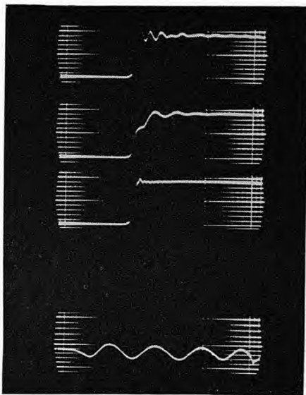
Figure 20. Same as figure 19, showing effect of long signal and ground leads
