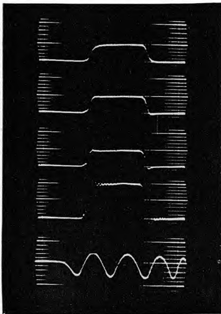
Figure 15. Resistance divider oscillogram
