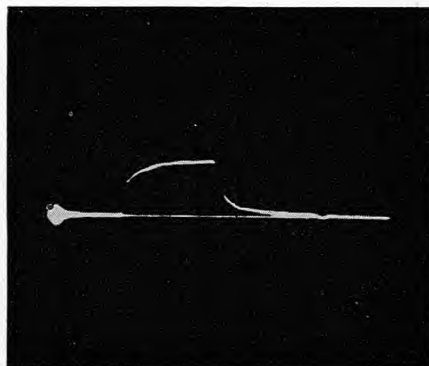
Figure 30. Microsecond response, long cable and no attenuator
