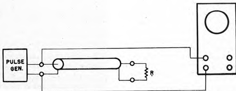
Figure 9. Typical setup for making line impedance measurements with pulses
