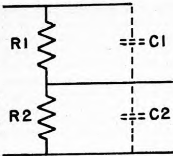
Figure 14. Attenuator circuit resulting from unbalancing stray capacitance
