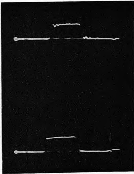
Figure 31. Microsecond response using RG-17/U cable
