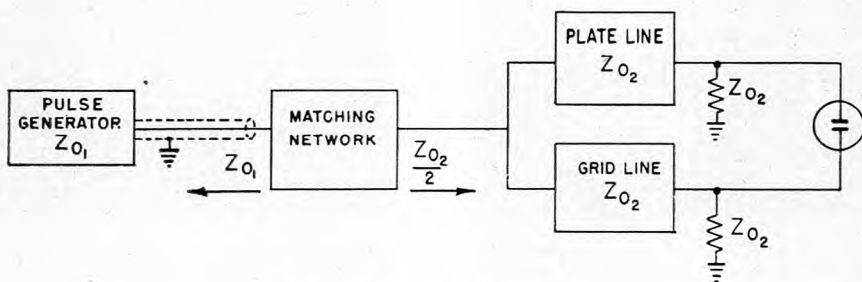
Figure 37. Cancellation setup
