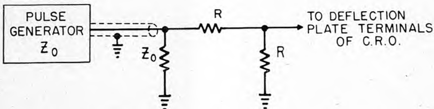
Figure 13. Circuit for studying effect of resistance dividers
