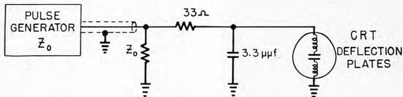
Figure 28. Circuit to compensate for deflection plate inductance
