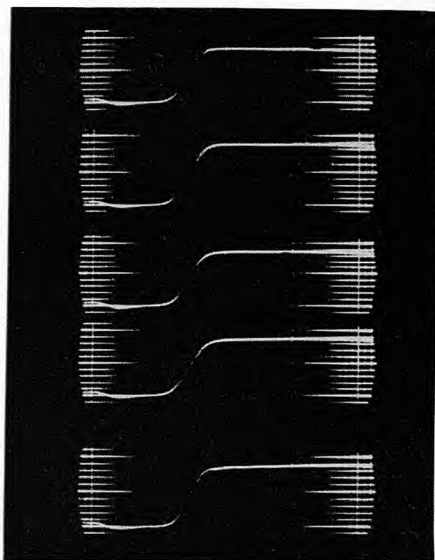
Figure 18. Oscillogram of a fixed attenuator test; using fast time base
