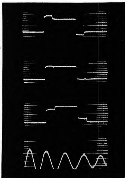
Figure 11. Oscillogram of line impedance measurements with long pulses
