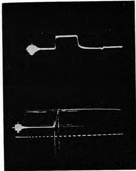
Figure 32. Pulse with a one millimicrosecond rise time
