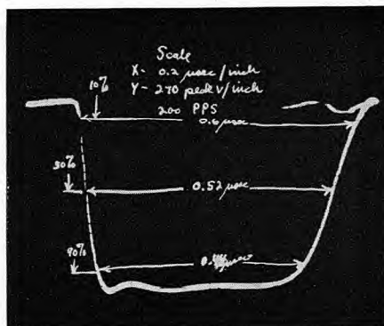
Figure 27. Same as figure 26, but using correct measuring techniques
