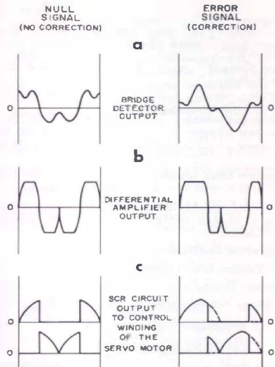
Figure 8. Waveforms present at the bridge detector, differential amplifier, and servo motor for no-error and error conditions. Note that servo action is based on position of zero crossings rather than on amplifier gain.
