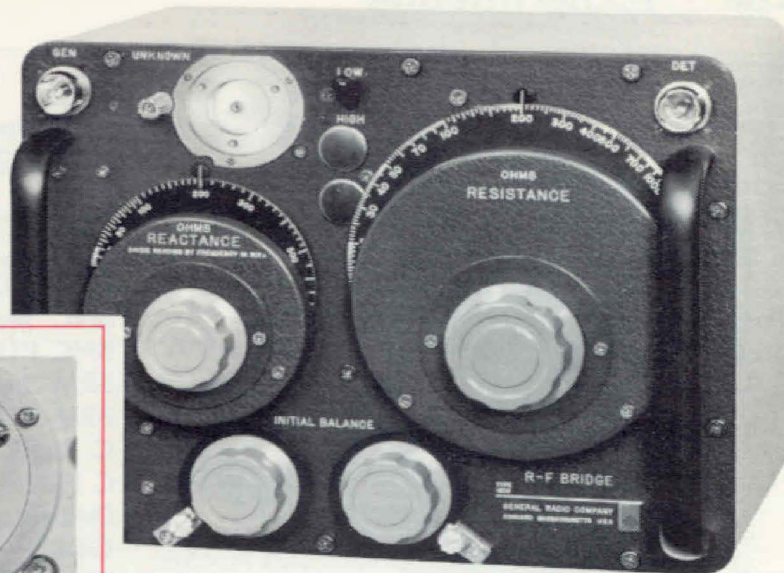
Figure 1. Type 1606-B RF Bridge. Inset shows GR900 ® adaptor in place.
