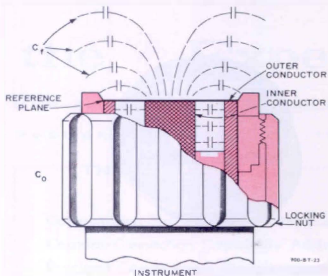
Figure 1. Open GR900® precision coaxial connector showing fringing capacitance ( C_f ).
