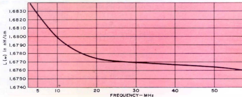
Figure 1. Typical inductance per unit length for Type 900-LB Precision Slotted Line.
