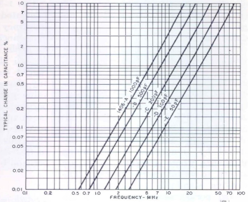
Figure 2. Typical percent increase in capacitance of Type 1406 Coaxial Capacitance Standards with frequency.
