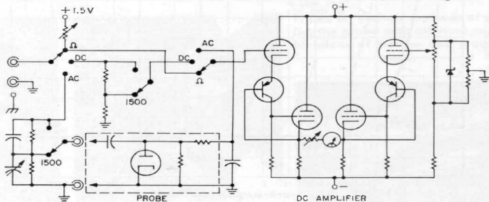
Figure 2. Simplified schematic diagram of the Type 1806-A Electronic Voltmeter.
