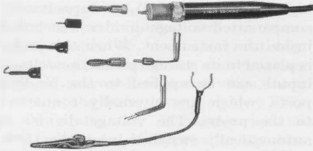
Figure 5. The ac probe and its accessory tips and ground clips.
