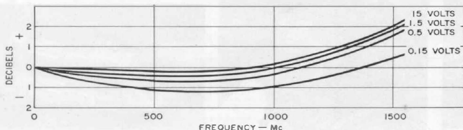
Figure 8. Typical high-frequency response characteristics of the probe and tee connector operating in a 50-ohm system.
