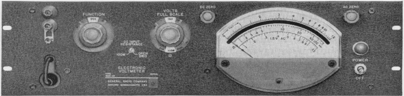
Figure 10. View of the Type 1806-AR Electronic Voltmeter for relay-rack mounting.
