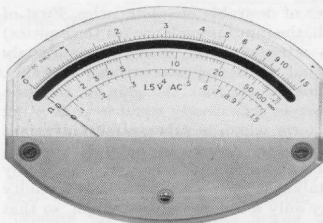
Figure 3. The meter scale. Note that all dc voltages and all ac voltages above 1.5 volts are read on a single scale.
