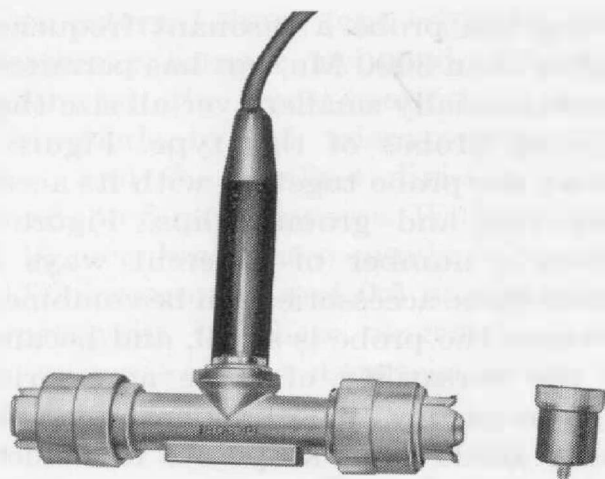
Figure 7. The probe with cap removed and the tee connector screwed on for ultra-high-frequency measurements.
