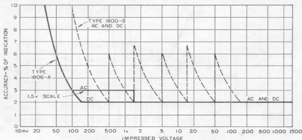
Figure 4. Accuracy as a function of scale reading for the Type 1806-A Electronic Voltmeter, compared with that of its predecessor, the Type 1800-B, whose accuracy was 2% of full scale.
