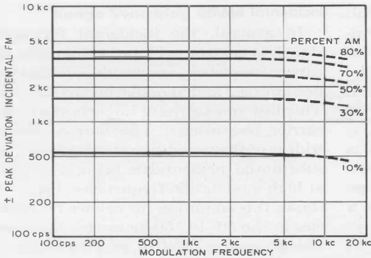
Figure 4. Incidental fm as a function of percentage modulation at high carrier frequencies.
