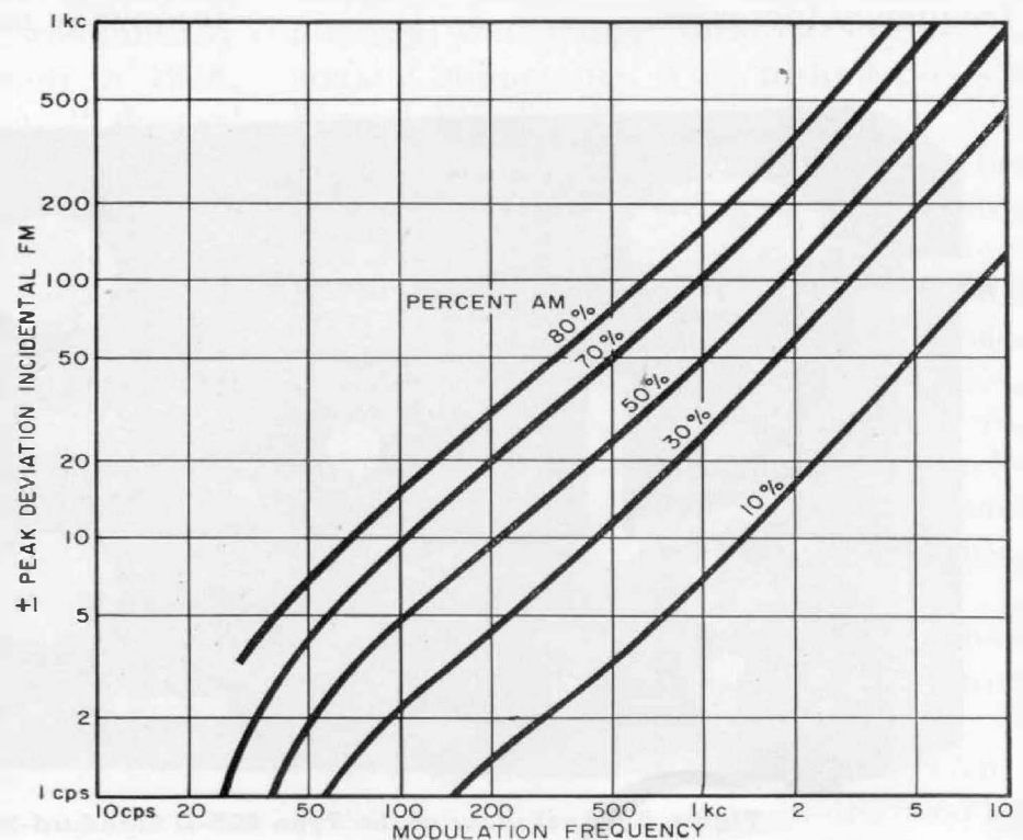
Figure 3. Incidental fm as a function of percentage modulation at carrier frequencies between 50 and 150 kc.
