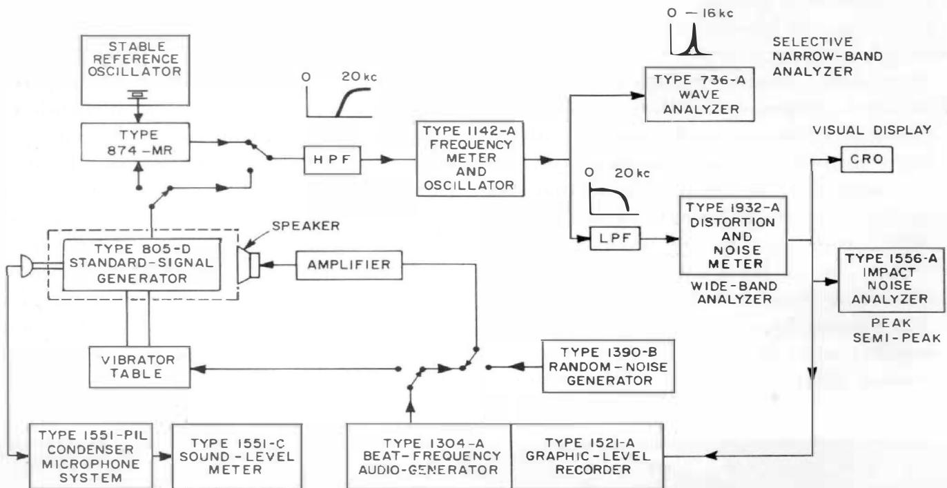
Figure 1. Block diagram of measurement system.
