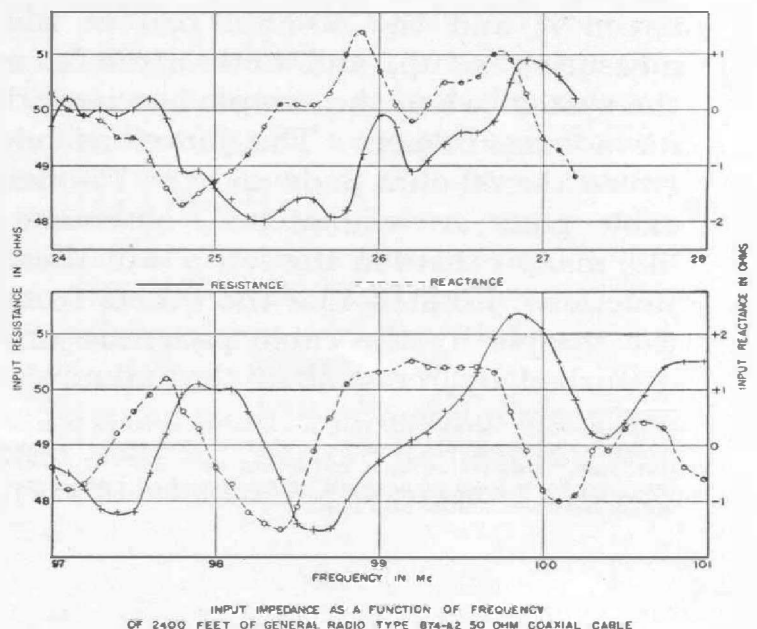
Figure 11. Input impedance as a function of frequency for 2400 feet of General Radio Type 874-A2 50-ohm Coaxial Cable.
