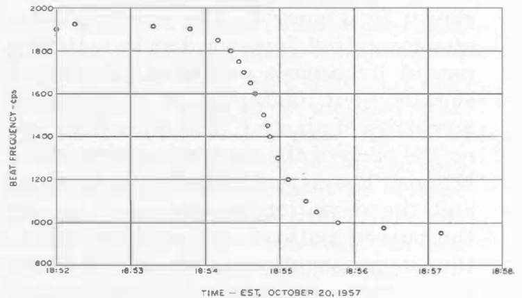
Figure 1. Measured frequency shift of signal from Sputnik I.
