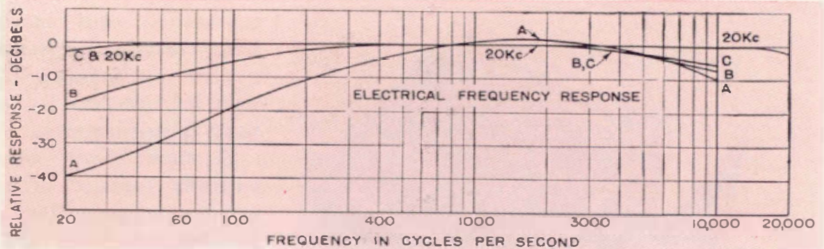
Figure 5. Frequency response for all positions of the weighting switch.
