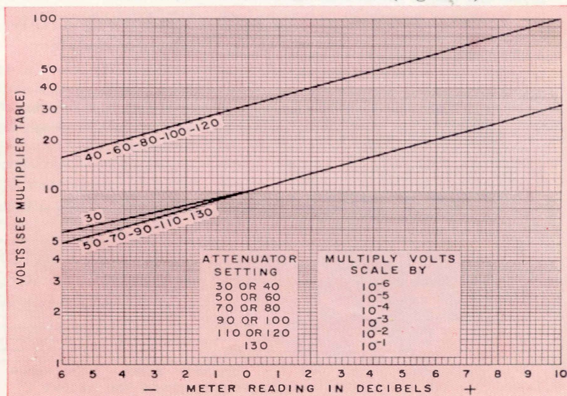
Figure 3. Chart for converting db readings to volts, after instrument has been standardized for full-scale values of 1, 3, 10, etc.
