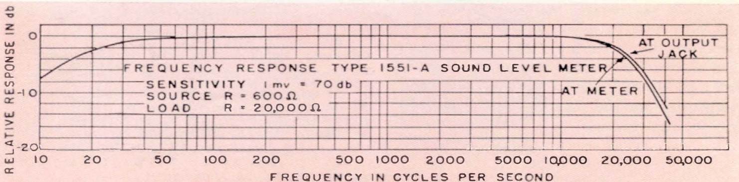
Figure 4. Over-all frequency characteristic, with weighting switch in 20 kc position.
