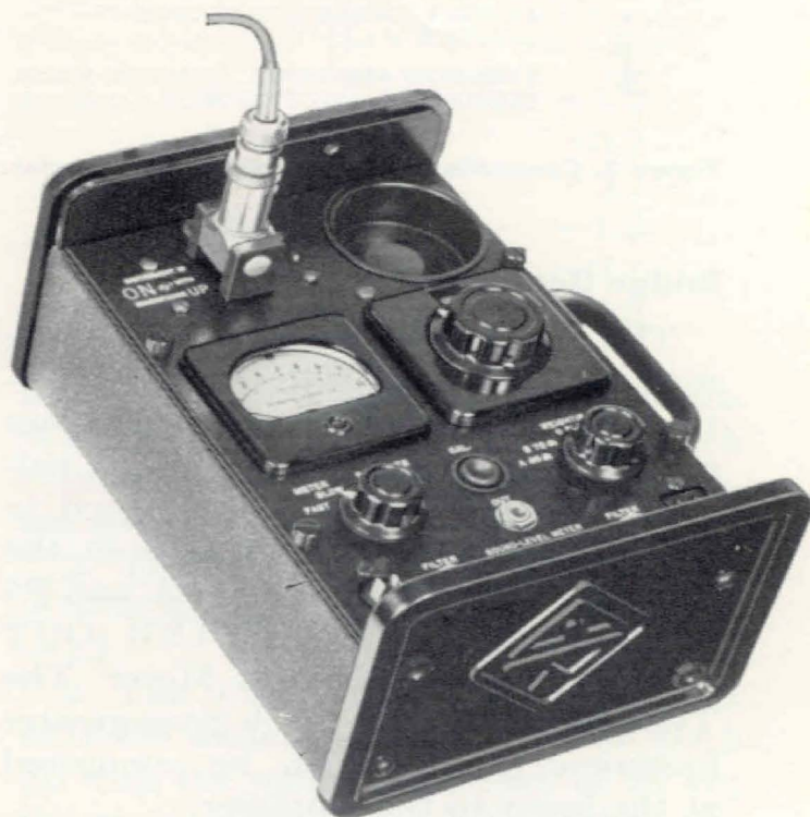
Figure 1. View of the Sound-Level Meter with microphone replaced by connector.
