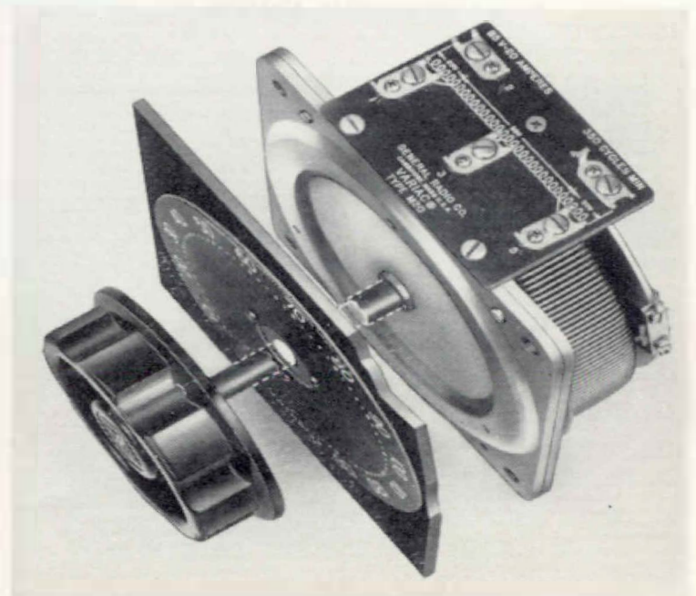
View of the Type M20 Variac.
