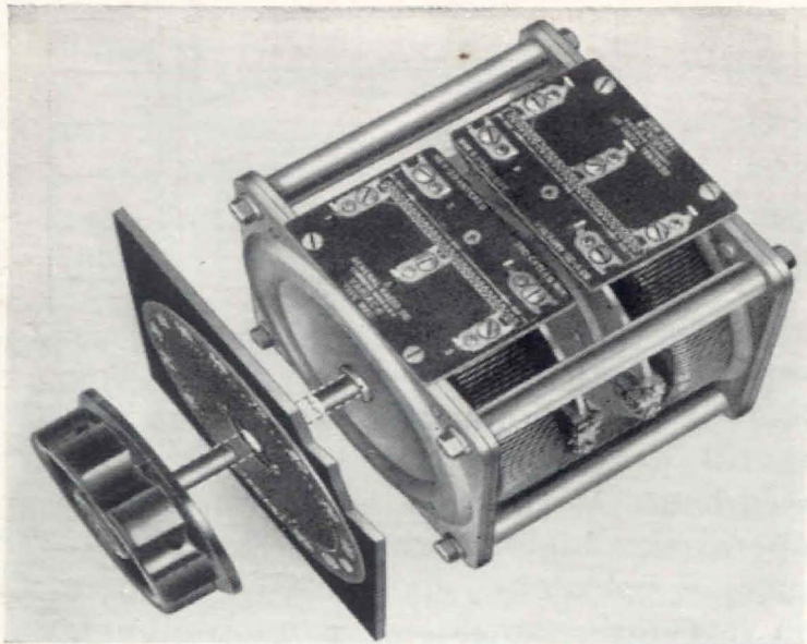
View of 2-gang unit, Type M20G2.
