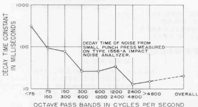
Figure 8. The time constant of analyzed noise from a punch press.
