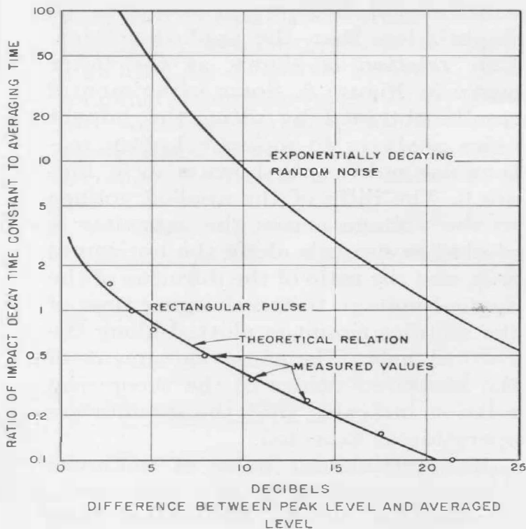
Figure 6. Chart showing the relations between the ratio of the peak to averaged value and the time constants of an impact and of the circuit. The lower curve is for a rectangular pulse, and the upper one is for the usual impact noises.
