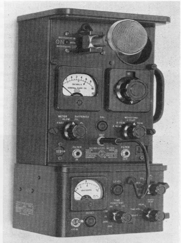
Figure 4. View of Impact Noise Analyzer attached to a sound-level meter.
