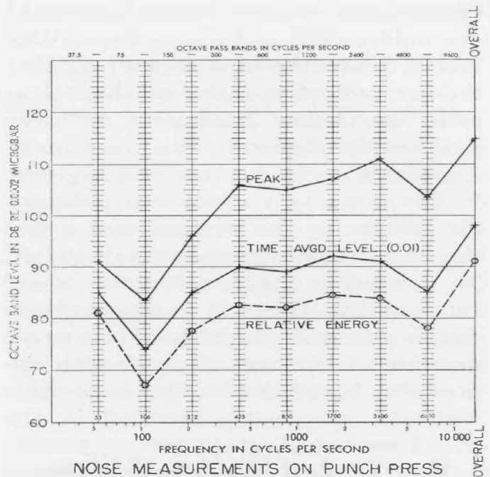
Figure 7. The results of an octave-band analysis of the noise from a single impact of a punch press as measured by the impact noise analyzer on the output of the octave-band analyzer.
