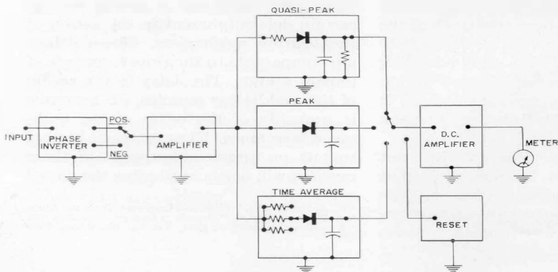
Figure 5. Simplified functional diagram of the Impact Noise Analyzer.
