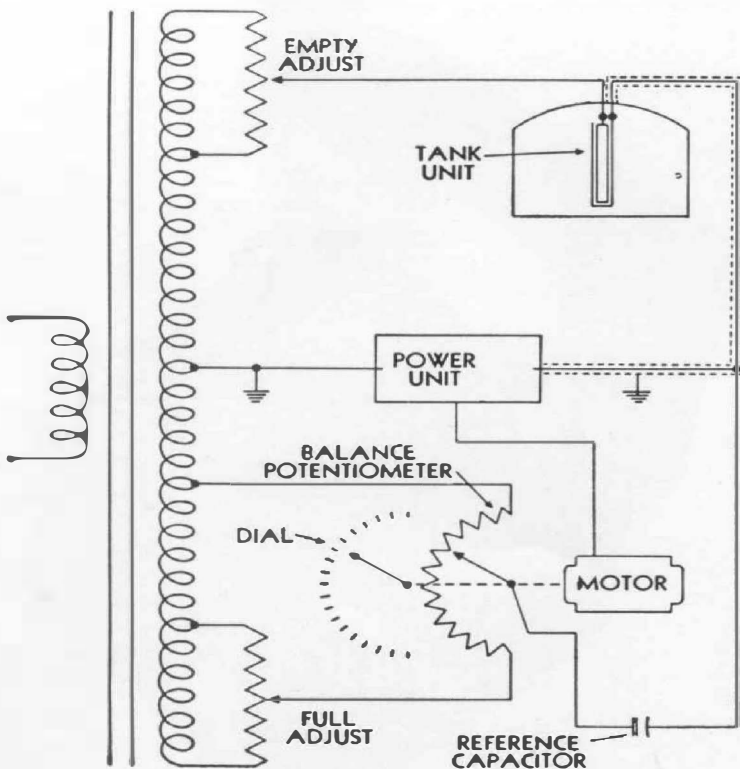
Figure 2. Schematic diagram of the capacitance null-type fuel gage, employing a self-balancing bridge. (Minneapolis-Honeywell)
