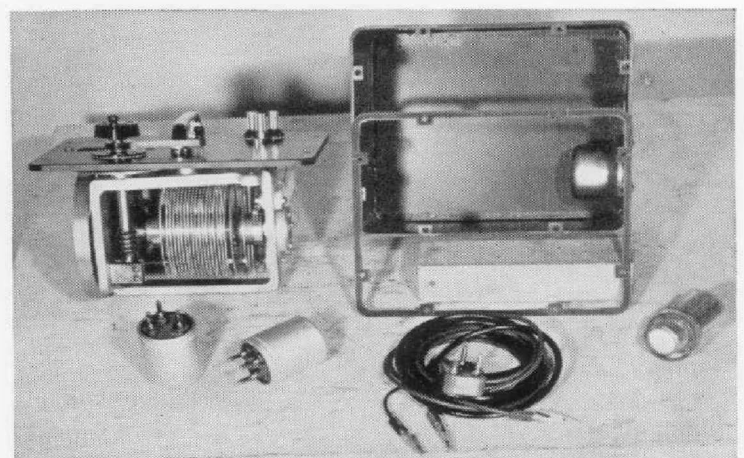
Figure 3. Elements supplied by the General Radio Company for the 0-3 Tester built by Minneapolis-Honeywell Regulator Company.
