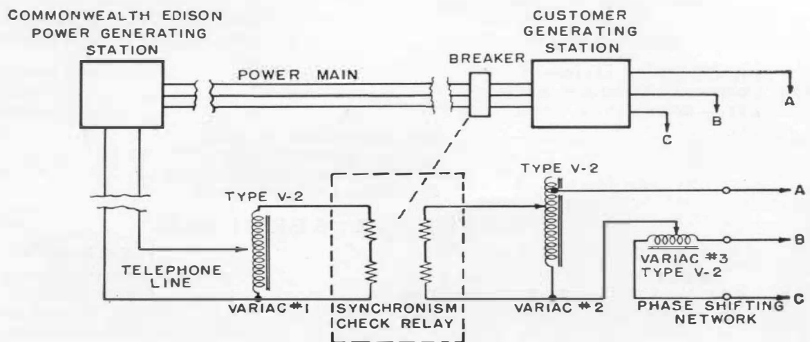
Functional diagram of the circuit used for phase monitoring.
