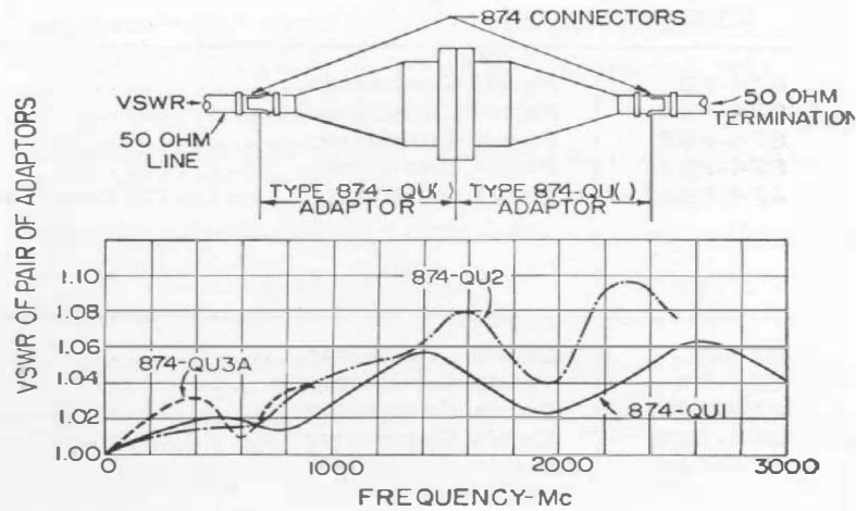
Figure 7. A plot of the VSWR as a function of frequency of pairs of adaptors from Type 874 Connectors to various sizes of 50.0-Ohm UHF Rigid Transmission Line.
