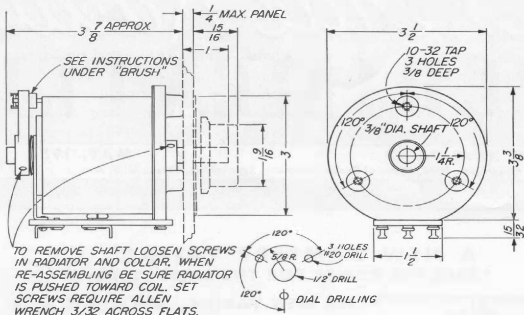
Figure 2. Dimensions of the Type V-2 Variac. Mounting dimensions and radial clearance are the same as for the older Type 200-B. Depth behind panel is slightly greater.
