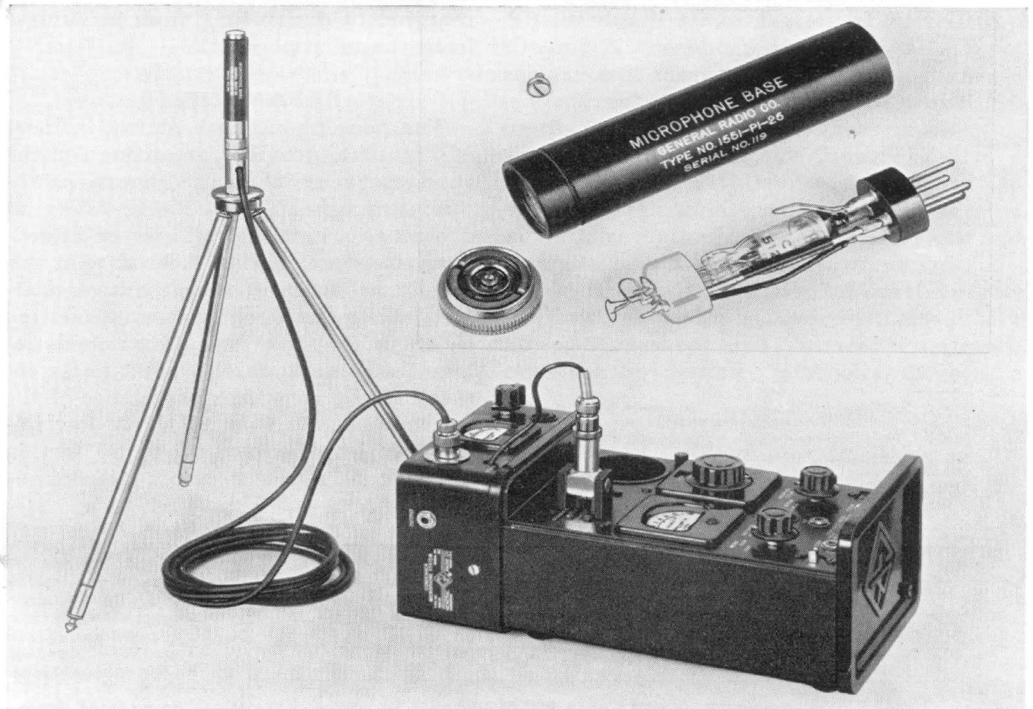
Figure 1. View of the Type 1551-A Condenser Microphone System attached to the Type 1551-A Sound-Level Meter. Inset shows microphone, microphone base, and preamplifier.
