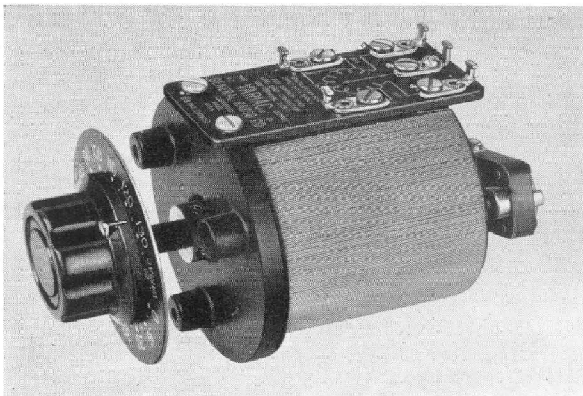
Figure 1. Designed for panel mounting, the new Type V-2 Variac Autotransformer gives more watts per dollar than its predecessor.
