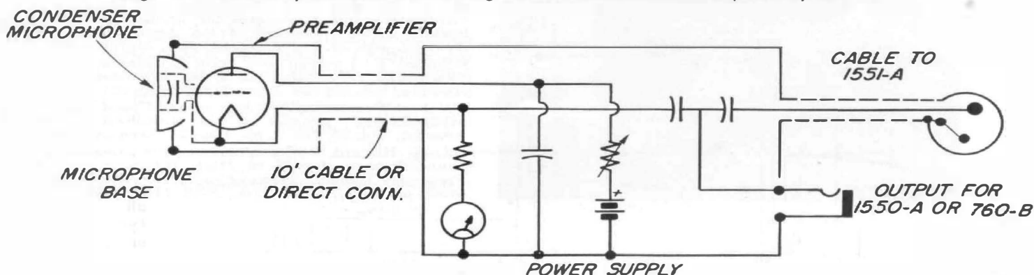
Figure 3. Elementary schematic circuit diagram of the condenser microphone system.
