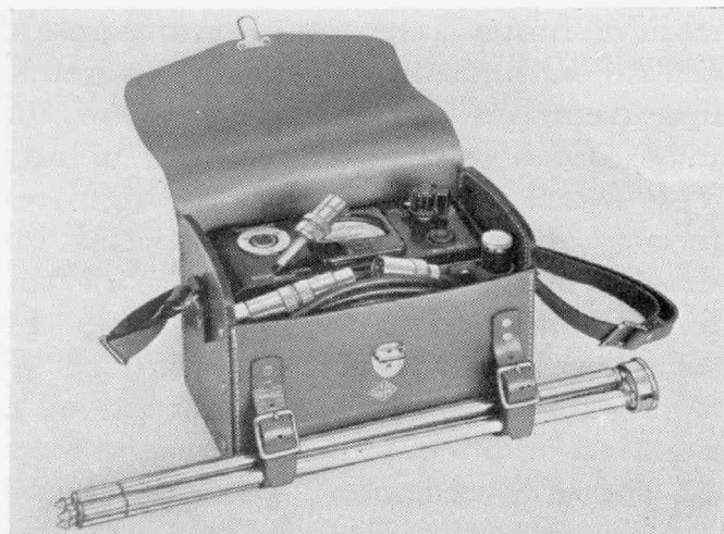
Figure 4. The condenser microphone system is furnished in a compact leather carrying case of top-grain cowhide.
