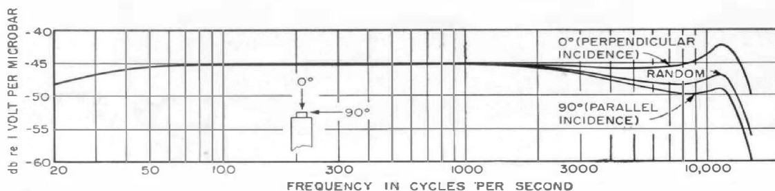
Figure 2. Frequency-response characteristics for different directions of incident sound. These characteristics show the overall response of the Type 1551-P1 Condenser Microphone System with the Type 1551-A Sound-Level Meter.
