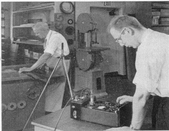
Figure 5. High-frequency sound, produced by a power saw, is measured with the sound-level meter and condenser microphone system.
