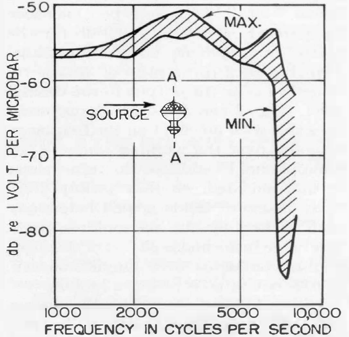
Figure 6. Variation in output of typical Rochelle salt crystal, diaphragm-type crystal microphone as a function of frequency as the microphone is rotated about axis A—A perpendicular to its diaphragm. Sound incidence is parallel to plane of diaphragm.
