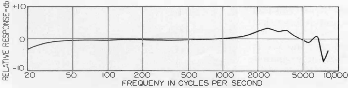
Figure 5. Typical response curve (random incidence) for sound-level meter and crystal microphone.
