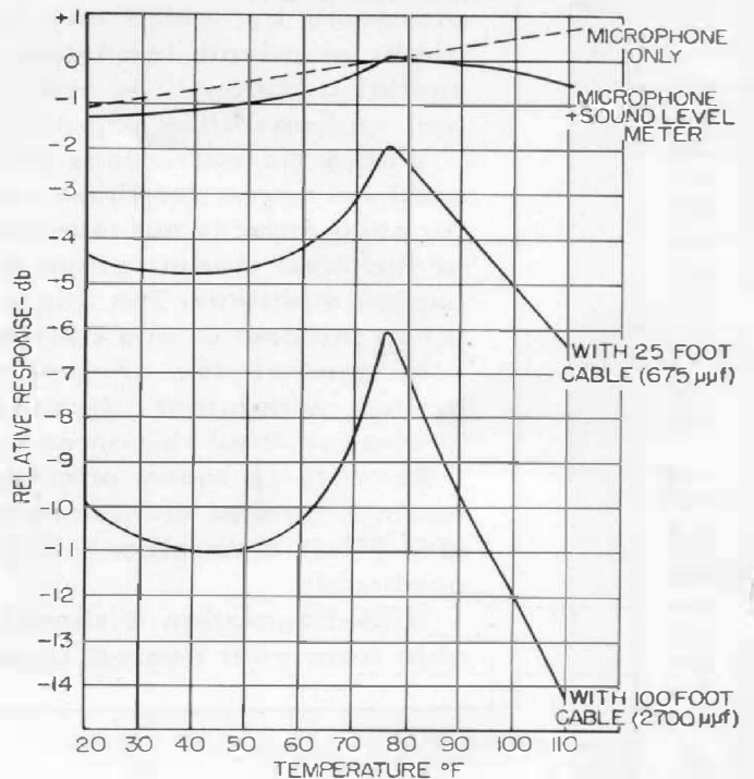
Figure 2. Variation in response as a function of temperature for the crystal microphone alone and with various lengths of cable between microphone and sound-level meter.
