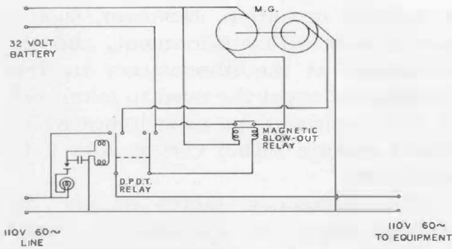
Figure 2. Schematic of the 32-volt d-c, 110-volt a-c motor generator set used in connection with each of the crystal clocks to provide emergency power with little delay. While a unit of this nature is capable of operating for a considerable time, limited only by the condition of the batteries, its main purpose is to provide a very quick source of 110 volts ac to tide over the short interval required for the gas-driven motor generator to build up.
