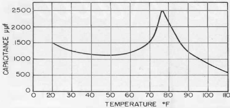
Figure 1. Capacitance variation as a function of temperature for a typical Rochelle salt crystal microphone.
