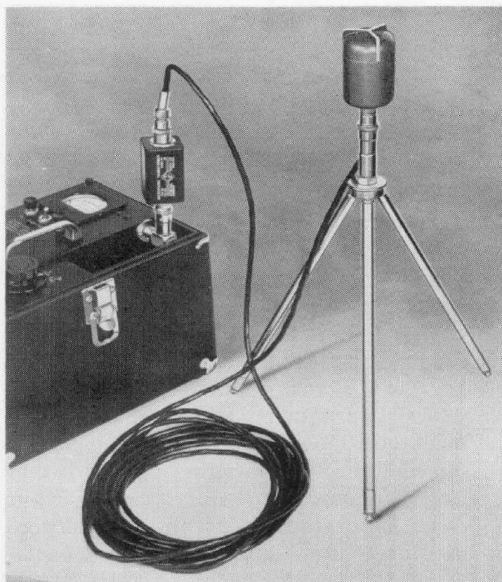
Figure 3. View of the Type 759-P25 Dynamic Microphone and Accessories connected to a Type 759-B Sound-Level Meter.
