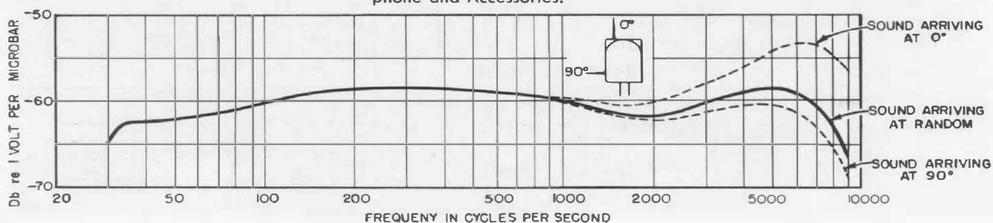
Figure 4. Typical response curves for the Type 759-B Sound-Level Meter with Type 759-P25 Dynamic Microphone and Accessories.
