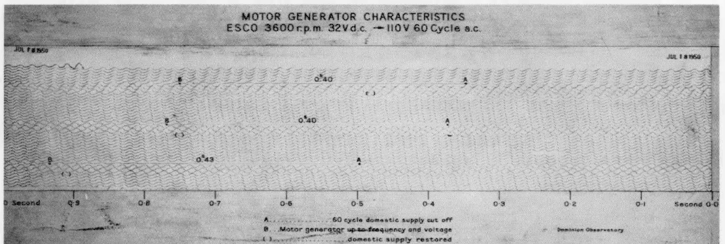
Figure 3. A recording on a drum which rotates at one revolution per second shows that the build-up time of the motor generator emergency power supply is less than half a second. The instant when the domestic power supply was cut off by pulling the switch is marked by A. The interval from A to B was required for the motor generator supply to build up to full frequency and voltage.
