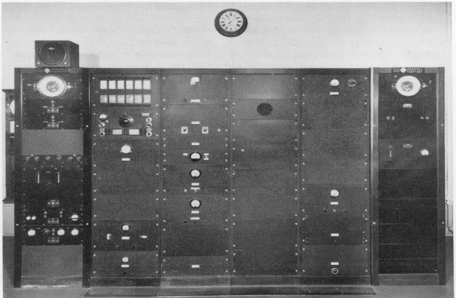
Figure 1. Bay of equipment in the Time Room at the Dominion Observatory. The two racks at either end contain the two General Radio Frequency Standards, or crystal clocks. The four racks in between contain a receiver, several relays and amplifiers, and the terminal blocks for the cables of wires which supply a multitude of services within the Observatory and to points outside.
