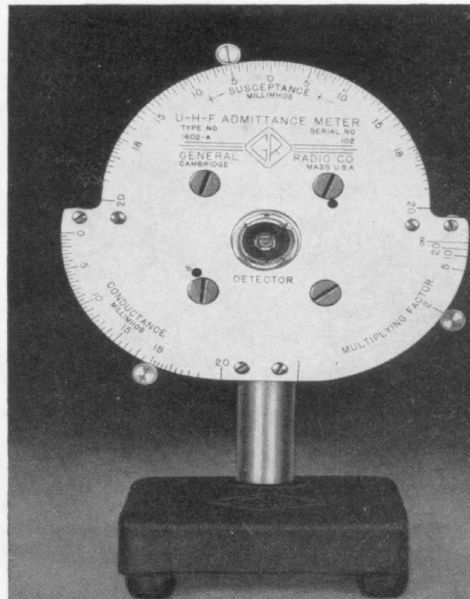
Figure 1. Front view of the Type 1602-A Admittance Meter, showing dial and sliding indicators. The extreme simplicity of operation is evident from this photograph. The indicators are moved along the scales until a null is obtained, and the conductance and susceptance are then read directly from the dial.
