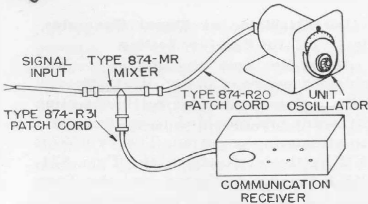
Figure 4. Functional diagram of the unit oscillator and mixer rectifier used as a frequency converter.
