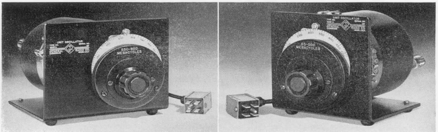
Figure 1. Panel views of the U-H-F and V-H-F Unit Oscillators. Left, Type 1209-A; right, Type 1208-A.
