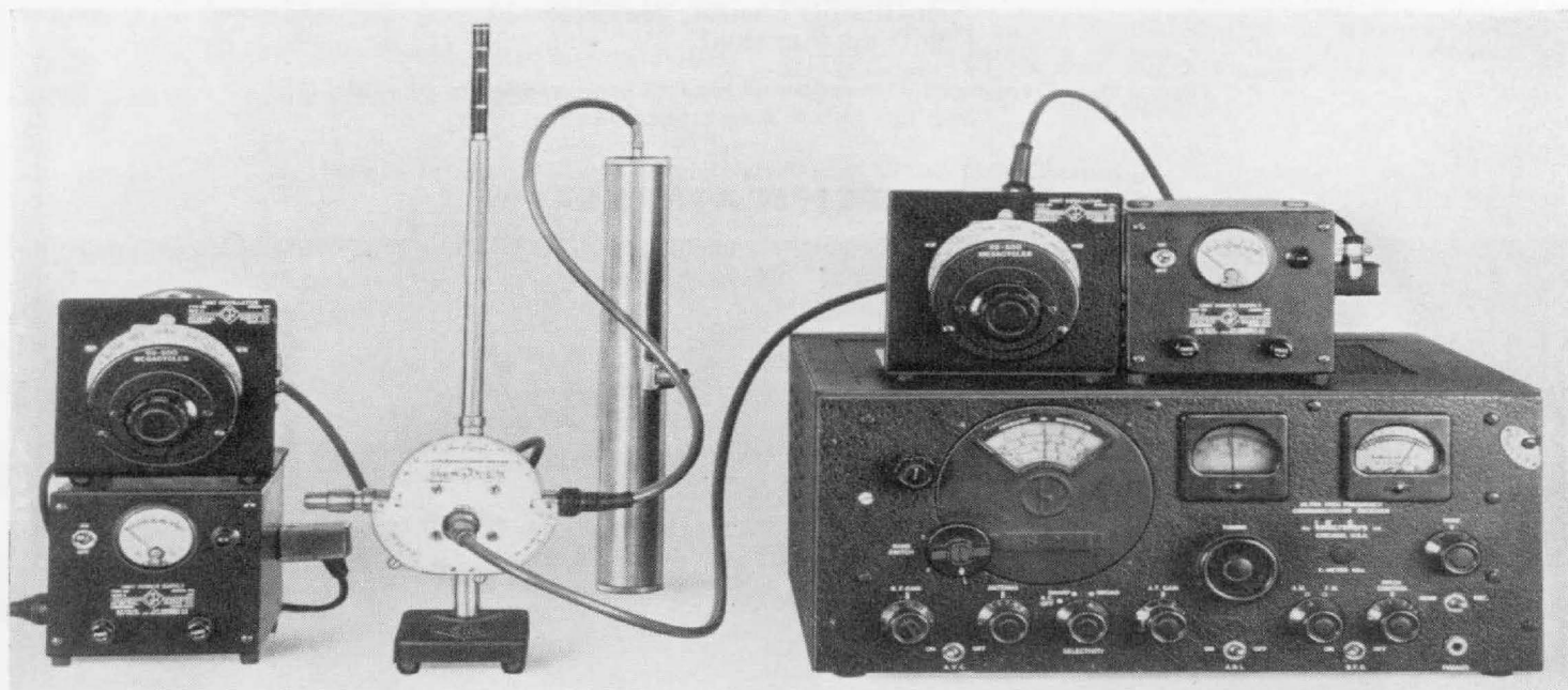
Figure 5. View of the admittance meter in use with standards and unknown connected. The generator is a Type 1208-A Unit Oscillator and the null detector is a communications-type receiver, with a second unit oscillator and Type 874-WM Mixer acting as a frequency converter. The unknown admittance being measured is an u-h-f transformer.
