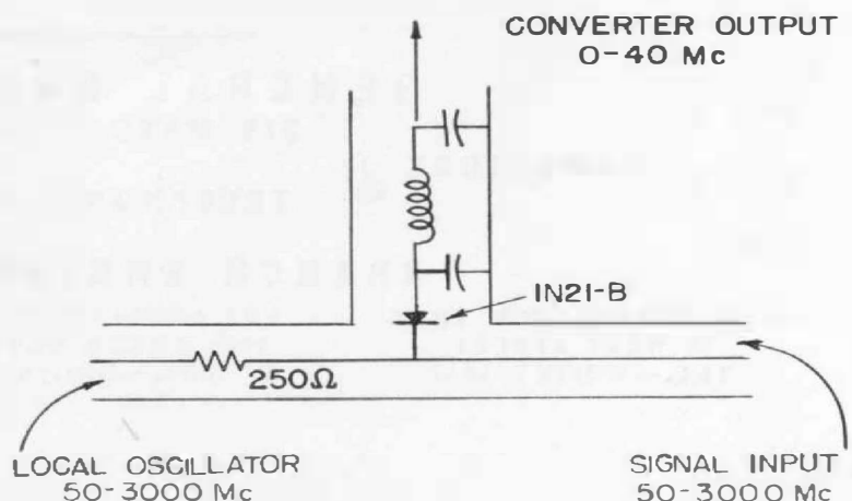
Figure 1. Schematic diagram of the Type 874-MR Mixer Rectifier.
