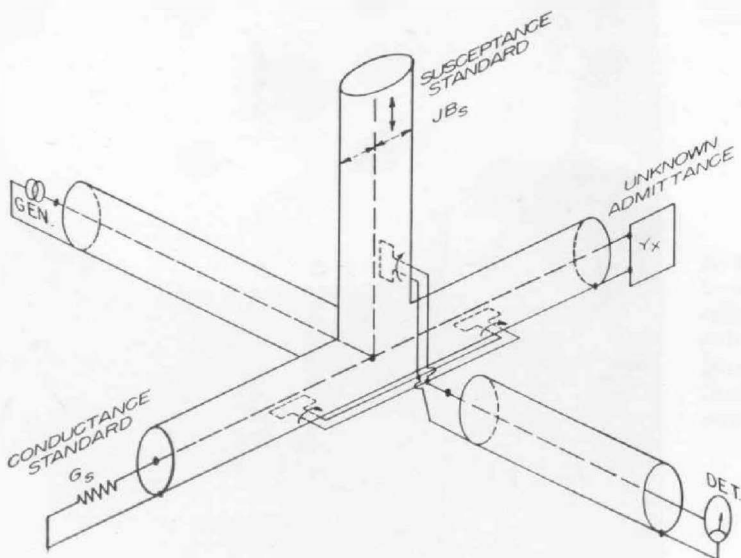
Figure 2. Schematic diagram of admittance meter circuit, with standards, generator, and null detector connected for admittance measurements.
