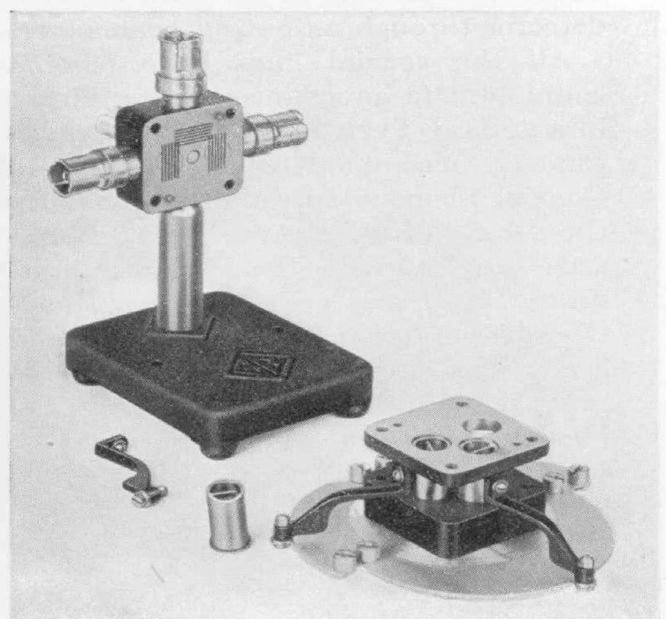
Figure 4. View showing internal parts of the admittance meter. The pickup-loop assembly has been removed from the generator junction assembly to show the coupling slots and the coupling loops.
