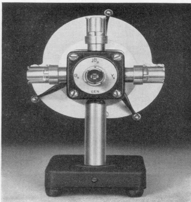
Figure 3. Rear view of the admittance meter, showing the four lines making up the generator junction assembly. The three arms for the sliding indicators can also be seen.
