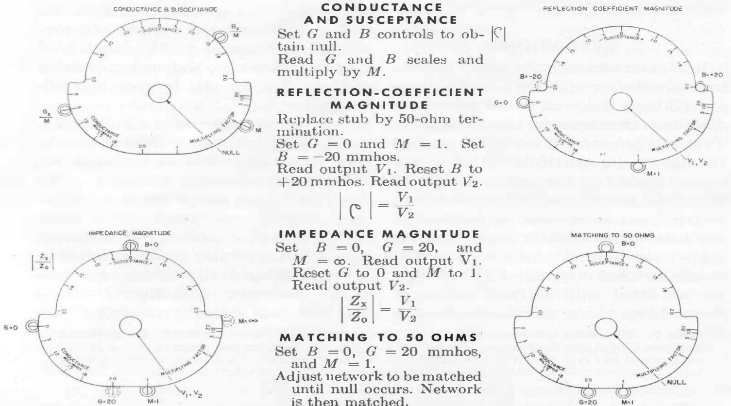
Figure 6. Graphical illustration of typical measurements possible with the U-H-F Admittance Meter.
