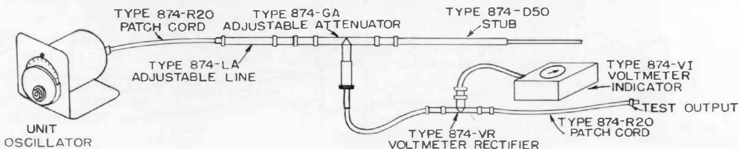
Figure 2. Functional diagram of the unit oscillator and accessories, connected to work as a standard-signal generator.
