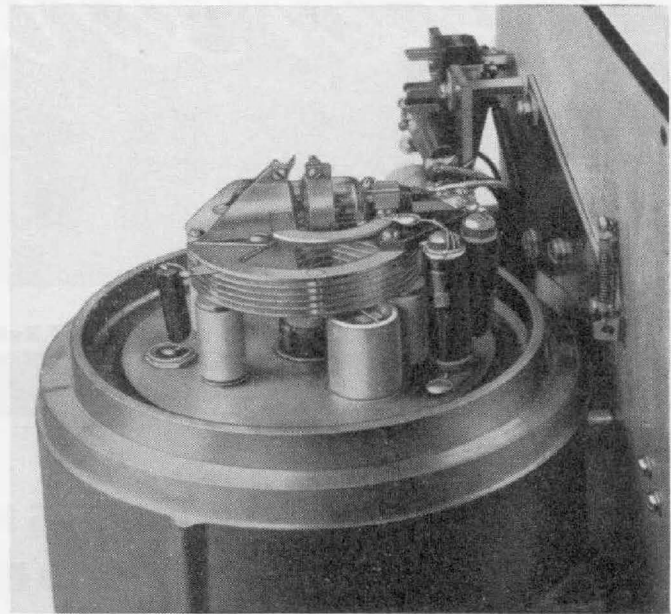
Figure 3. View of the oscillator portion of the U-H-F Unit, with cover removed from casting to show tube, butterfly, and attenuator input.
