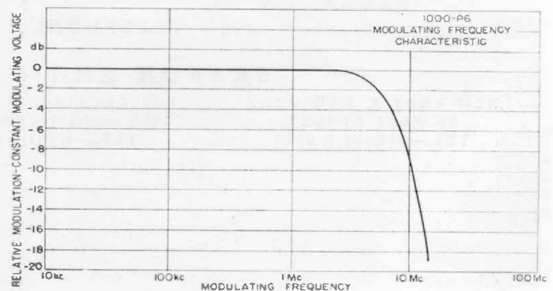
Figure 3. Modulating frequency characteristic.
