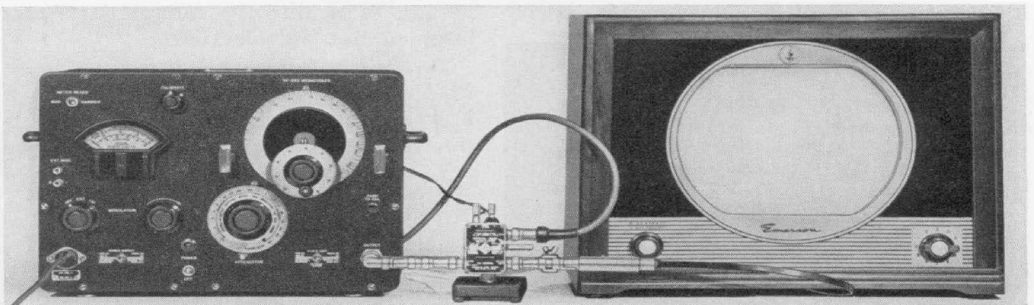
Figure 5. The Type 1021-AV V-H-F Standard-Signal Generator with Type 1000-P6 Crystal Diode Modulator, set up for tests on a television receiver.
