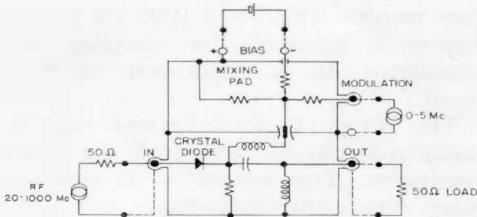
Figure 2. Circuit of the modulator.
