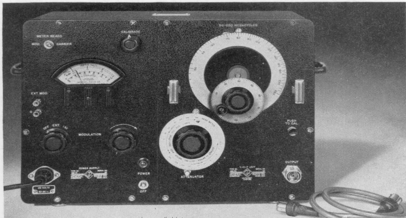
Figure 1. Panel view of the Type 1021-AV V-H-F Standard-Signal Generator.
