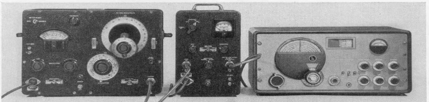
Figure 5. The Type 1021-AV V-H-F Standard-Signal Generator and the Type 1023-A Amplitude Modulator, arranged for tests on a communications-type receiver.
