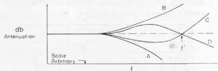
Figure 7. Extension of high frequency range by compensation.
