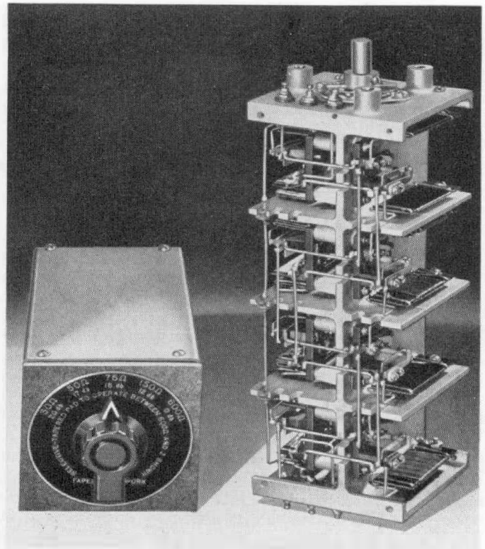
Figure 10. (Left) Type 829-HT Decade Attenuator Unit (tapered model) and (right) typical internal construction of the Type 829 Decade Attenuator Units.
