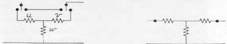
Figure 2. Elements of a T-pad, u and v series elements, w shunt element.
