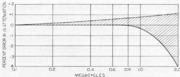
Figure 9. Maximum limits of frequency discrimination in compensated Type 829-TA, -TB, -TC Units.
