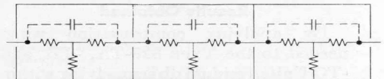
Figure 4. T-pads in single shield compartments.
