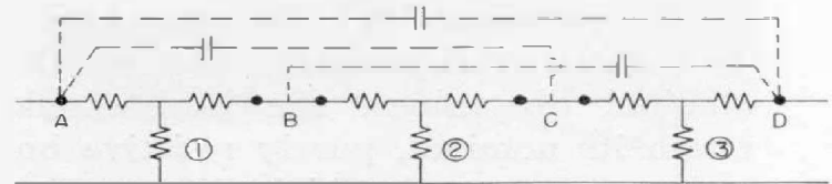
Figure 3. High-frequency cross-talk in a series of T-pads without shields.
