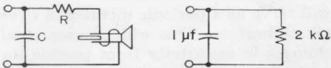
Figure 2. Electrical circuit (left) and equivalent circuit (right) of the Sound-Level Calibrator.
