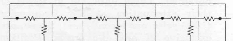
Figure 5. T-pads in bisected shield compartments.
