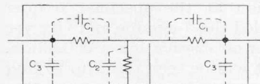
Figure 6. Unavoidable residual capacitances, T-pad with bisected shield.
