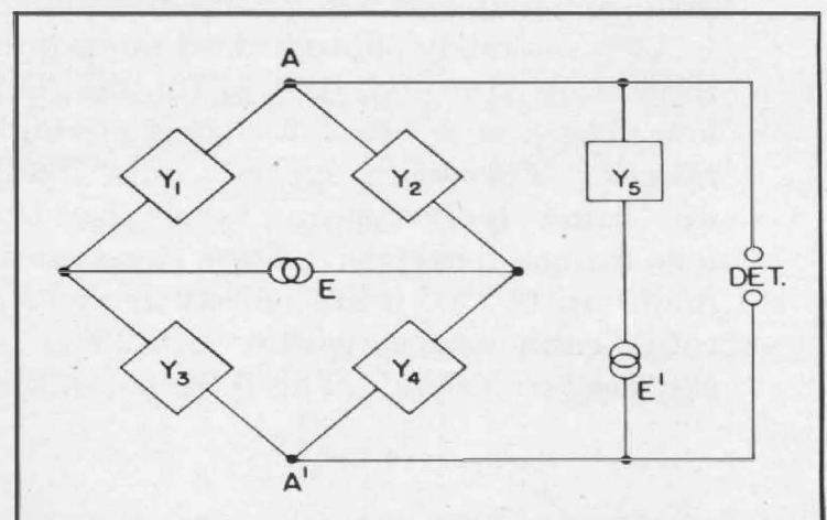
Figure 6. Equivalent circuit of the bridge and compensating circuit.
