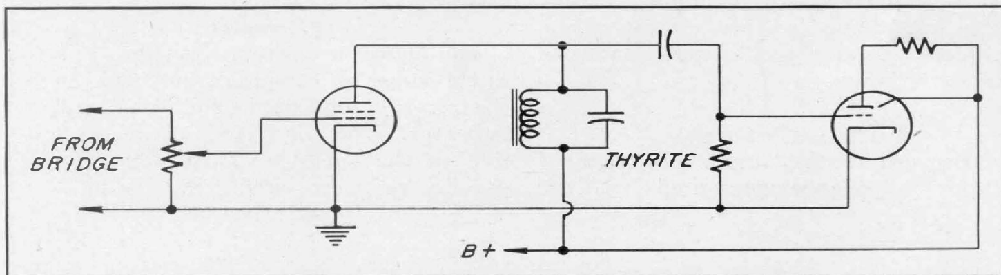
Figure 4. Elementary schematic diagram of the null detector.
