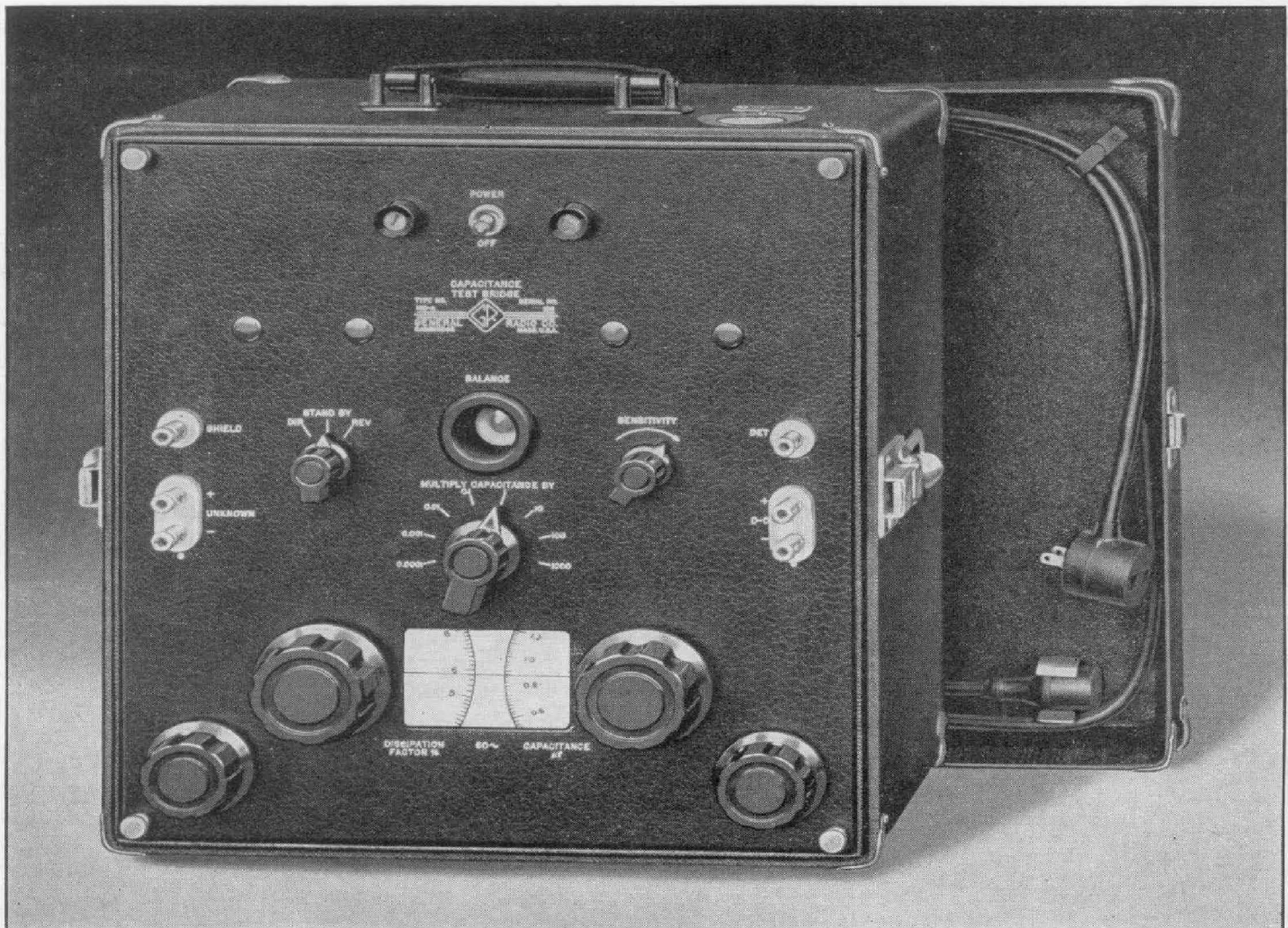
Figure 1. Panel view of the Type 1611-A Capacitance Test Bridge with cover of cabinet removed.
