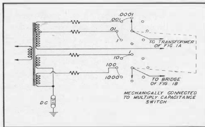
Figure 3. Arrangement of power supply switching to obtain the maximum safe power for each multiplier position.
