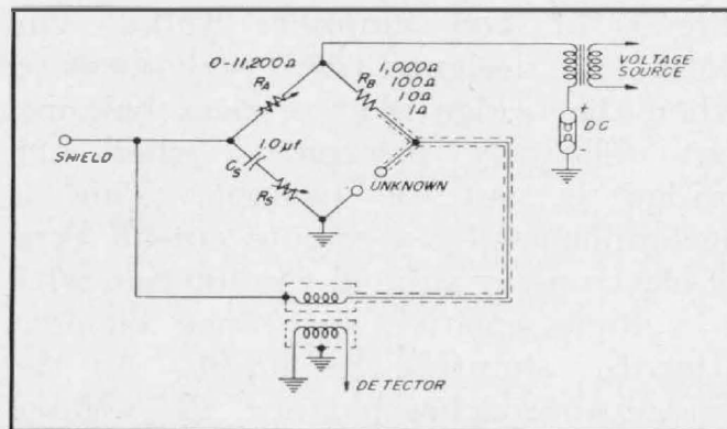
(Left) Figure 2a. Basic bridge circuit used for the four lower multiplier positions.
