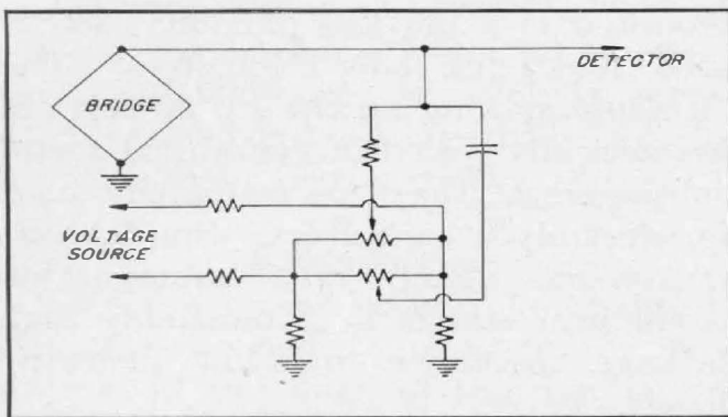
Figure 5. Schematic diagram of circuit used to cancel the unbalance voltage produced by the zero capacitance.
