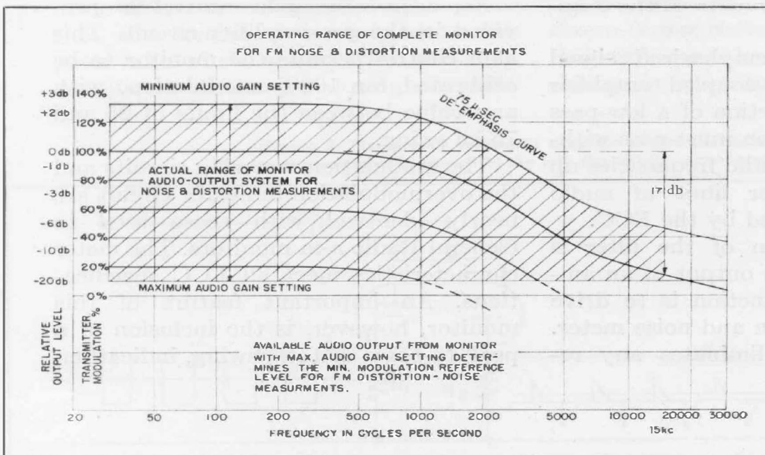
Figure 4. Operating range of the monitor for distortion and noise measurements.
