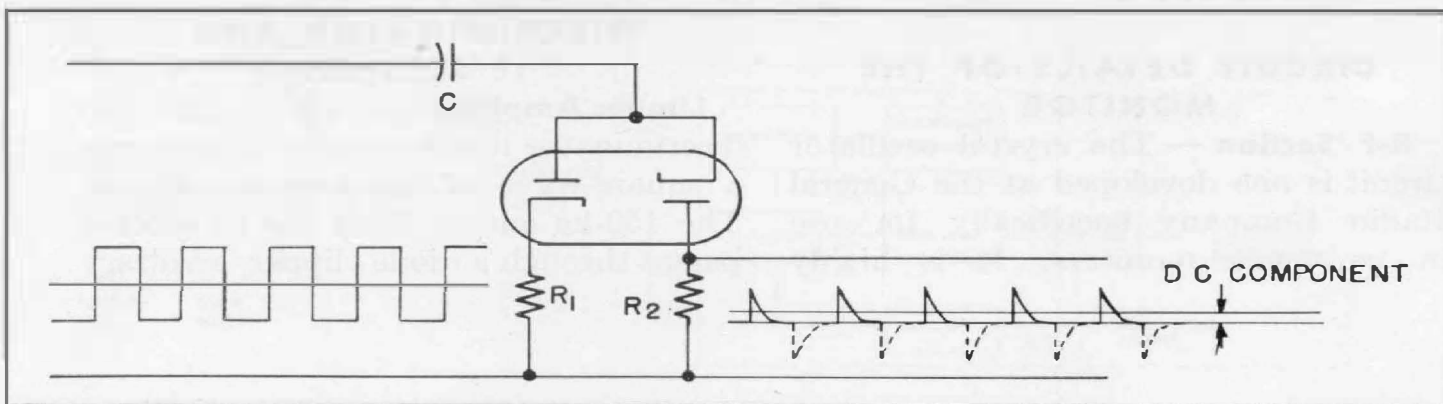
Figure 3. Elementary schematic diagram of the discriminator. The input waveform is shown at the left, the output waveform at the right.
