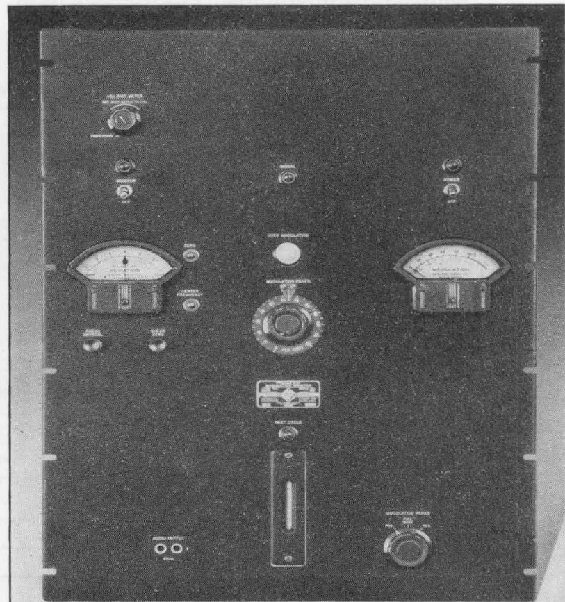
Figure 1. Panel view of the Type 1170-A F-M Monitor.
