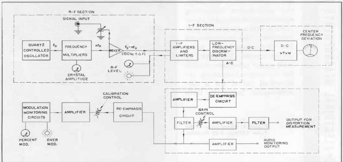
Figure 2. Functional block diagram of the monitor.
