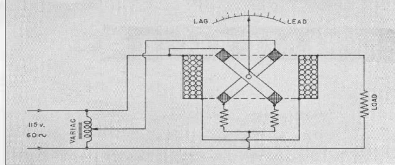
FIGURE 4. Diagram showing how the Variac is connected to the power-factor meter. With connections as shown, one-half the scale can be calibrated. By shifting the Variac to the other movable coil, the other half of the scale can be covered.
