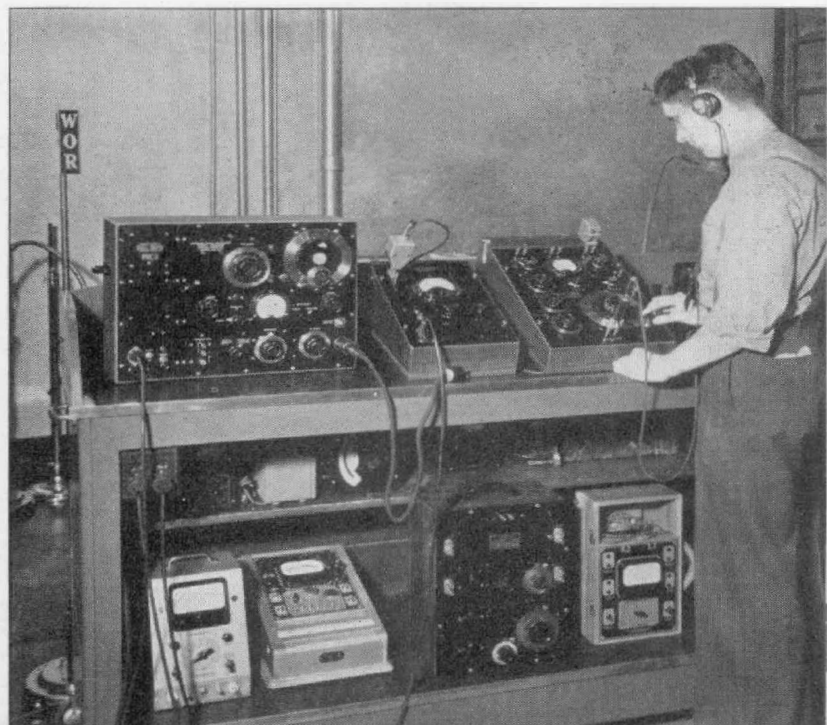
FIGURE 4. Another view of the test bench showing the TYPE 650-A Impedance Bridge in use.
