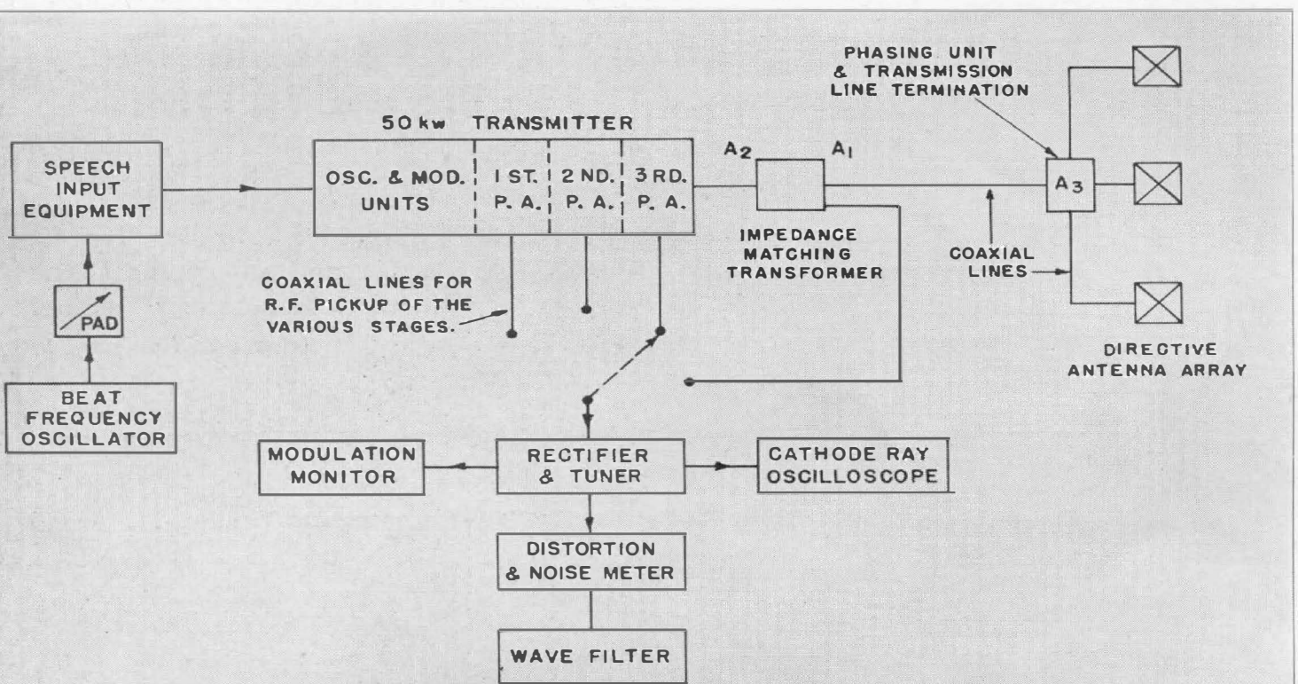
FIGURE 1. The arrangement of equipment for routine modulation, distortion and noise tests at WOR. Coaxial lines from each power amplifier stage are brought to the measurements room and permit measurements to be made on individual stages. Antenna impedance is measured at A 1 , A 2 , and A 3 .
