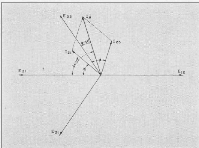
FIGURE 3. Vector diagram of the voltage and current relations in the three-phase power-factor meter. The current through the fixed coil is I_A , and the voltages across coils B and C are E_{21} and E_{23} respectively.
