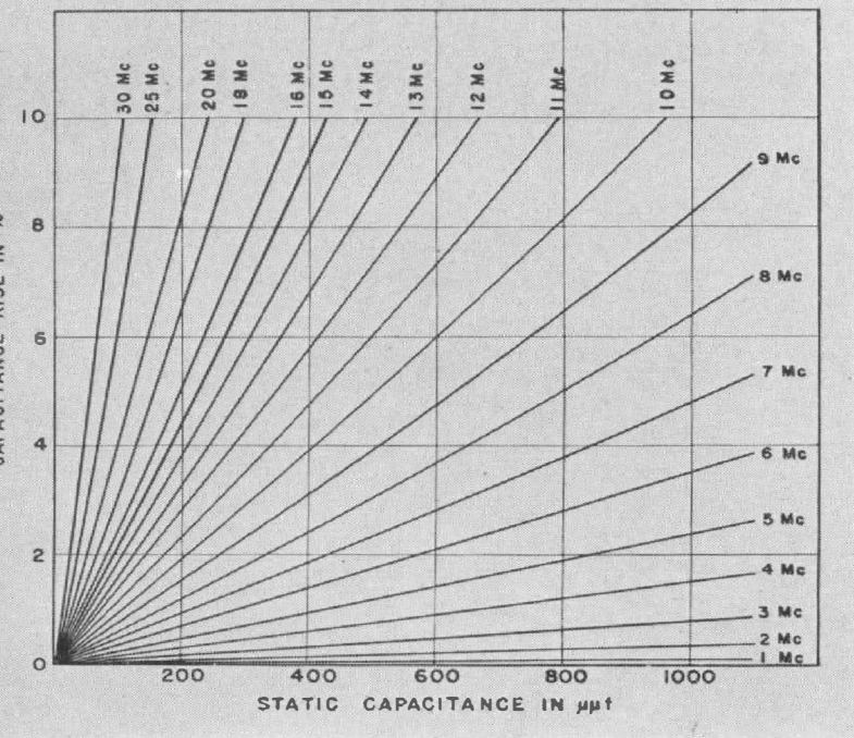
FIGURE 6. Variation in effective capacitance of TYPE 722-N Condenser as a function of static capacitance for various frequencies.
