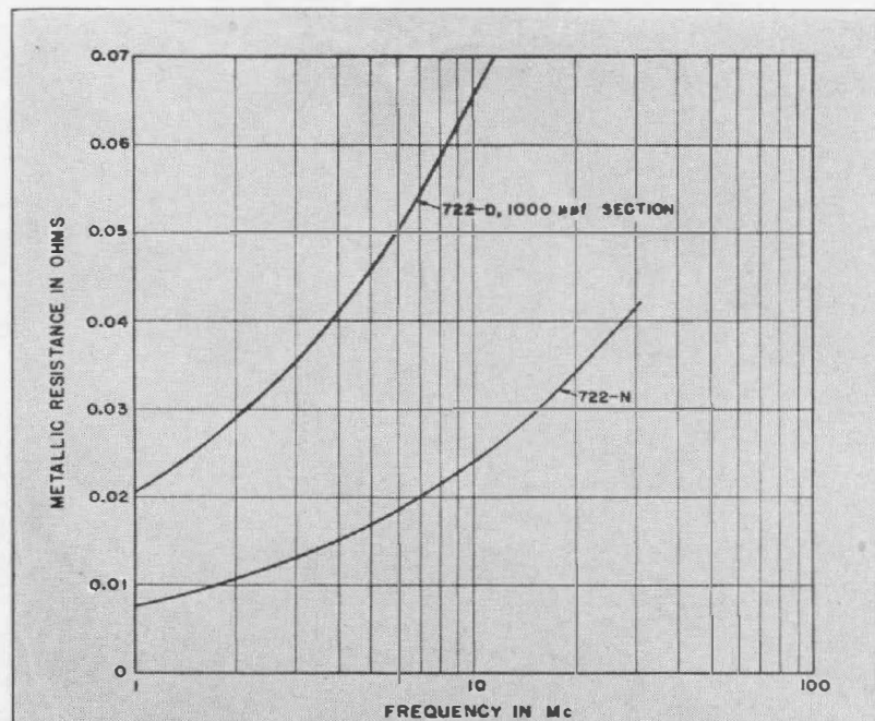
FIGURE 5. Metallic resistance of Type 722-N Precision Condenser as a function of frequency. For purposes of comparison, the resistance of TYPE 722-D is also shown.
