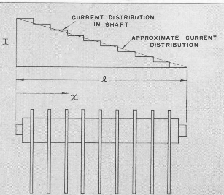
FIGURE 3. Showing the distribution of current in a rotor shaft fed at the left-hand end.
