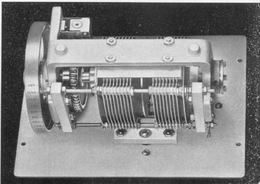
FIGURE 1. Interior view of the TYPE 722-N Condenser showing the method of feeding the rotor. For a close-up view of the brush mechanism, see page 6.
