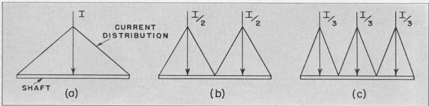
FIGURE 4. Current distribution when current is fed symmetrically to the shaft.
