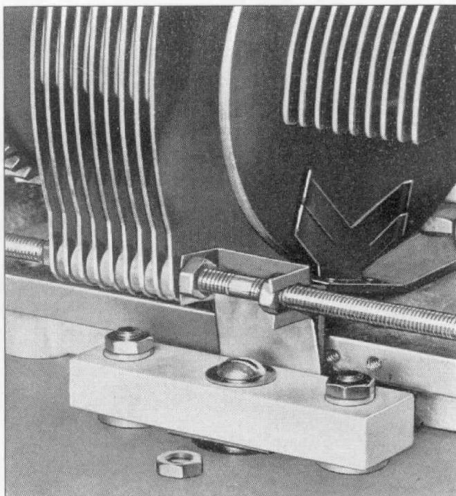
FIGURE 7. Showing the leads and the method of connection to the rotor.
