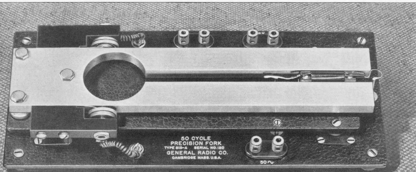
FIGURE 1. Photograph of TYPE 815-A Precision Fork.
