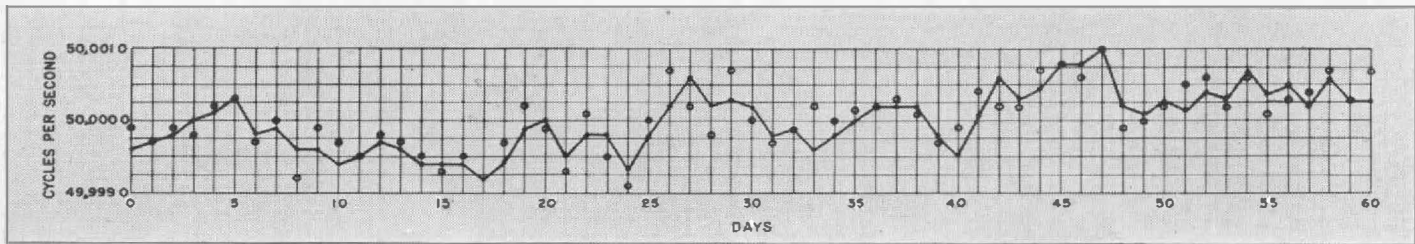
FIGURE 2. Plot of the results of a 60-day test run on TYPE 815-A Precision Fork.
