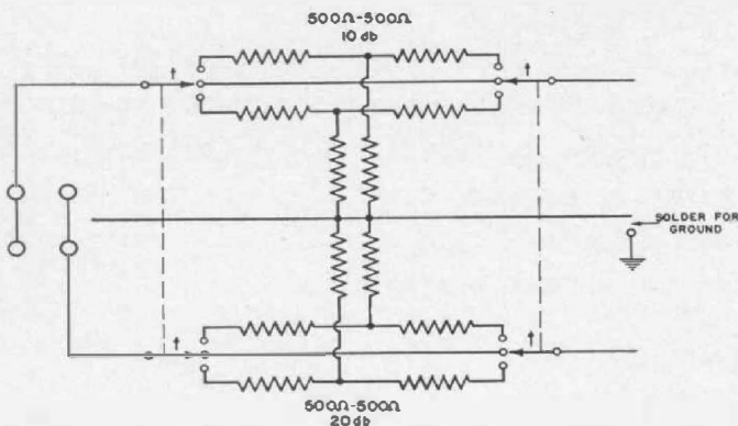
FIGURE 2. Wiring diagram of the first switch. Connections for the other two switches are similar
