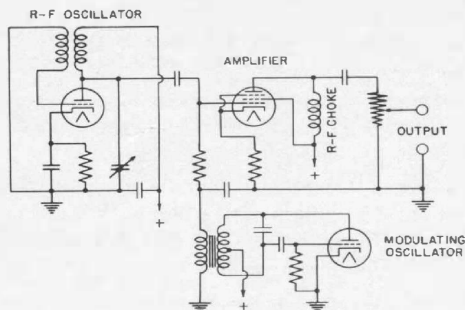
FIGURE 3. Schematic wiring diagram of TYPE 684-A Modulated Oscillator. For the sake of simplicity, power supply connections are omitted, as are the 1000-cycle output terminals and the modulation switch and its associated terminals for using the 1000-cycle oscillator tube as a detector
