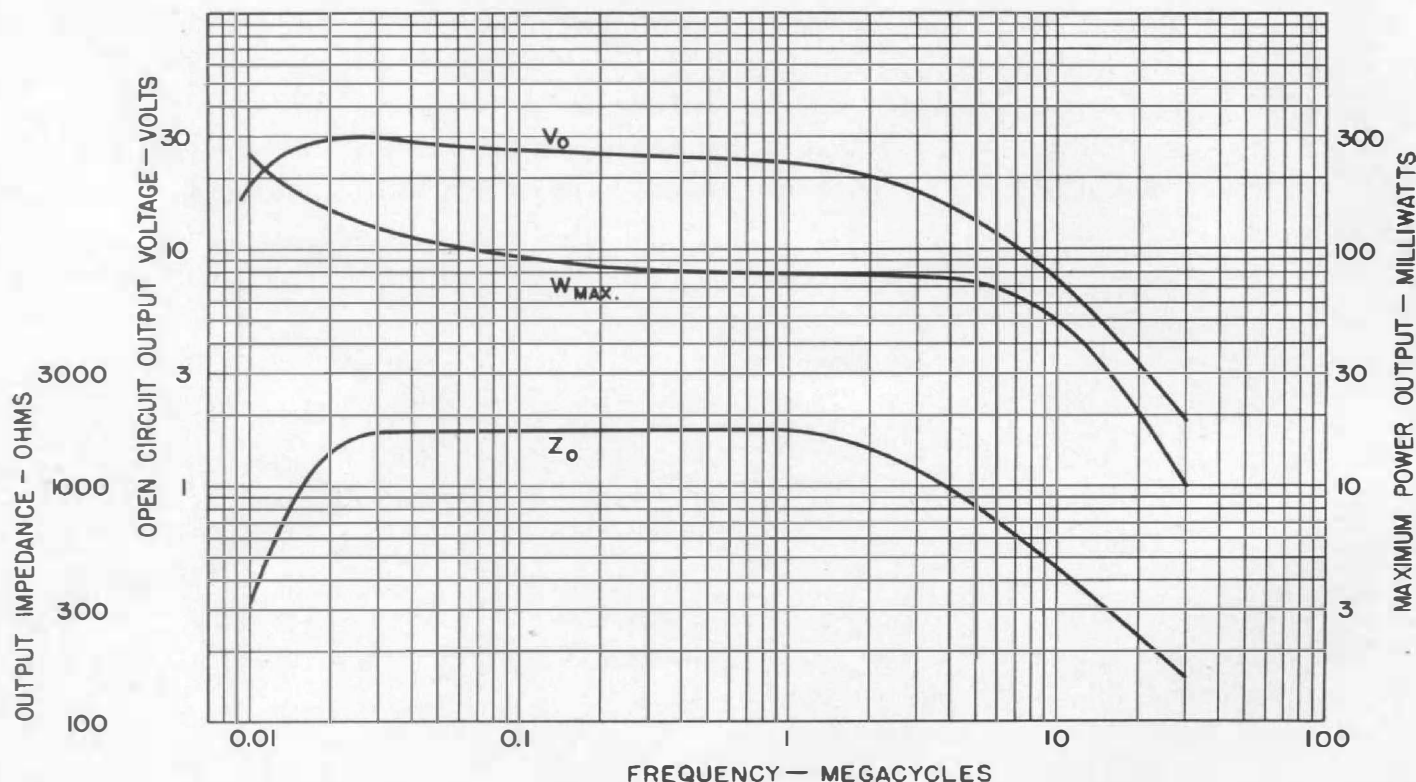
FIGURE 2. Output characteristics of the modulated oscillator. The power curve shows the maximum obtainable into a resistive load. These are average curves and do not take into account the slight differences in voltage and power which occur between the high-frequency end of one range and the low-frequency end of the next range at the same frequency
