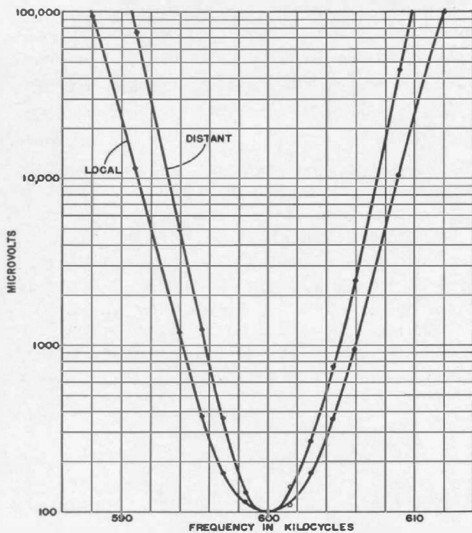
FIGURE 3. A selectivity curve for a radio receiver, taken with the TYPE 605-B Standard-Signal Generator
