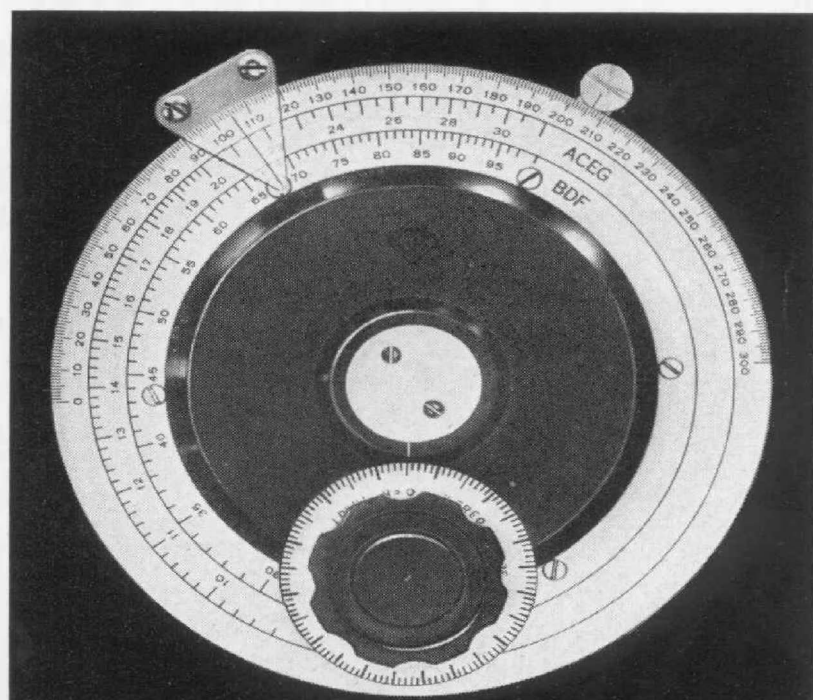
FIGURE 2. Photograph of the main and auxiliary dials. These are also used on TYPE 684-A Modulated Oscillator
