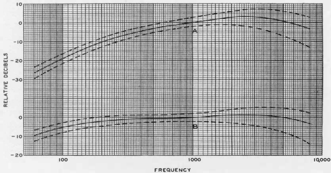
FIGURE 2. Frequency characteristics specified by the A.S.A. Curves A and B are respectively the so-called 40 db and 70 db equal-loudness contours modified to take account of the differences between random and normal free-field thresholds. Allowable tolerances are shown by the broken lines. These same tolerances are allowed on a flat characteristic
