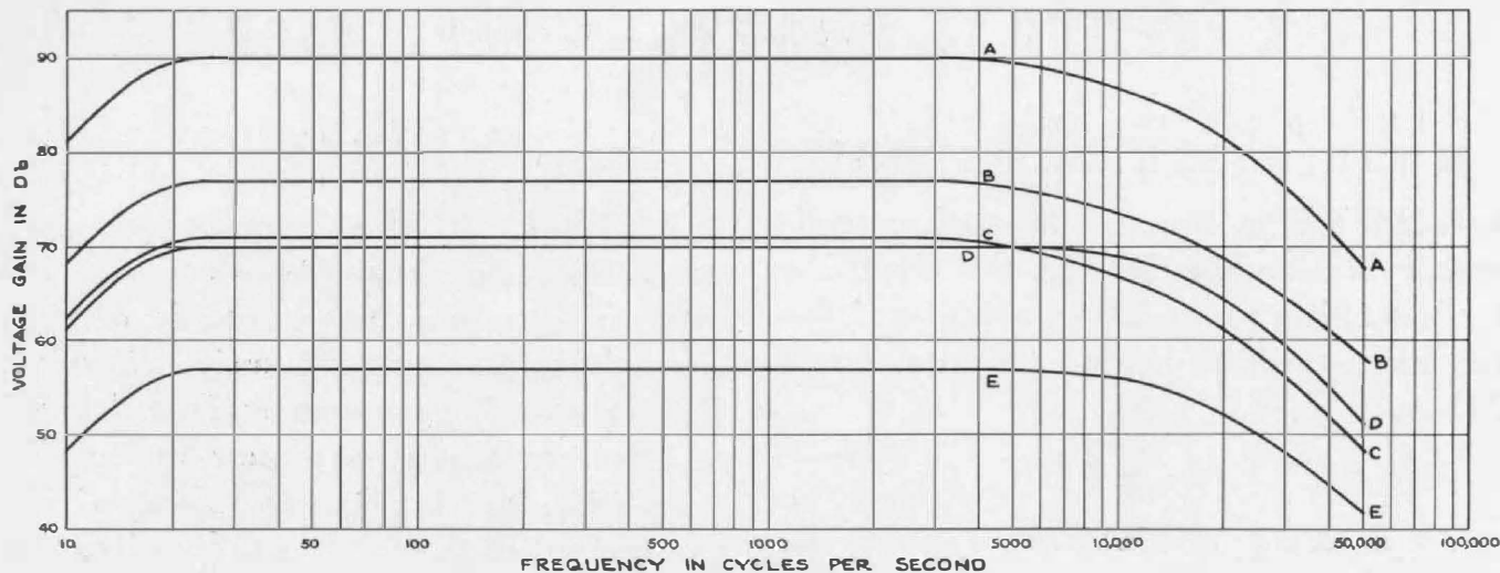
FIGURE 2. Frequency characteristics of TYPE 814-A Amplifier under various load conditions. Curves A and B were taken with loads of 1 megohm and 20,000 ohms respectively with the INPUT VOLTAGE switch in the LOW position. Curves D and E were taken with the same loads, but with the switch on HIGH. Curve C is the same as Curve B but with the GAIN control turned down 6 db
