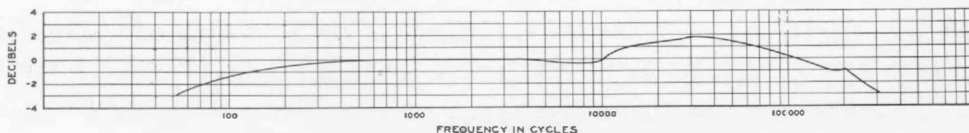
FIGURE 2. Frequency characteristic TYPE 741-J Interstage Transformer. Voltage ratio 1 : 1
