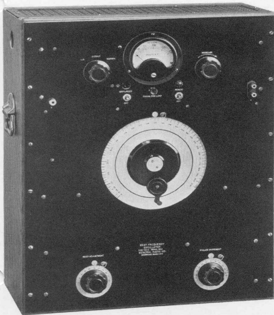
The TYPE 713-A Beat-Frequency Oscillator. A new a-c operated oscillator with undistorted output of 2 watts. The frequency range is 10 cycles to 16,000 cycles.
