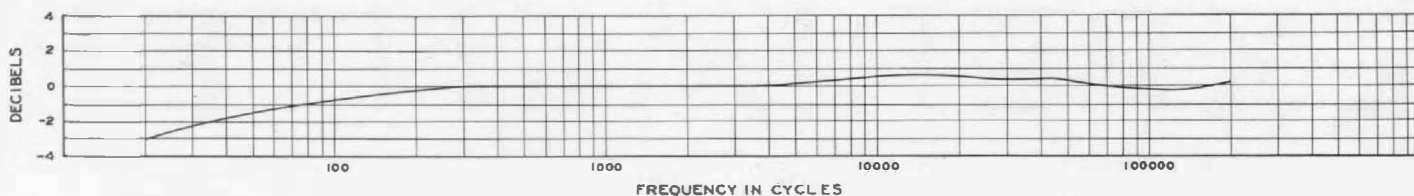
FIGURE 1. Frequency characteristic TYPE 741-G Line-to-Grid Transformer. Voltage step-up ratio 1 : 6.4
