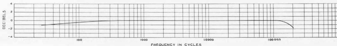
FIGURE 3. Frequency characteristic TYPE 741-P Plate-to-Line Transformer. Voltage step-down ratio 6.35 : 1
