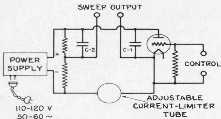
FIGURE 2. Schematic diagram for the TYPE 655-A Bedell Sweep Circuit
