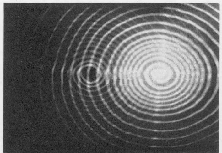
Two maximum-velocity spirals of the type described in the accompanying article. Each was taken with a different accelerating voltage on the tube
