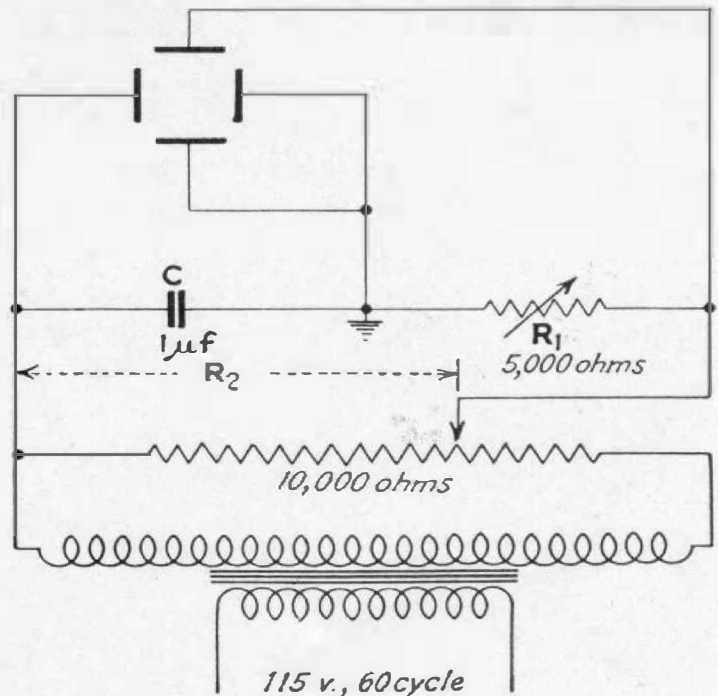
Circuit for measuring the maximum velocity of oscillograph spot that a given lens-emulsion combination will record
