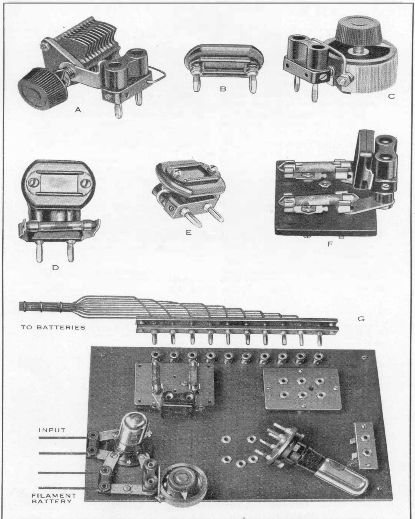
A few common plug-in circuit components, easily built up from standard TYPE 274 Plugs, Jacks, and Mounting Bases
