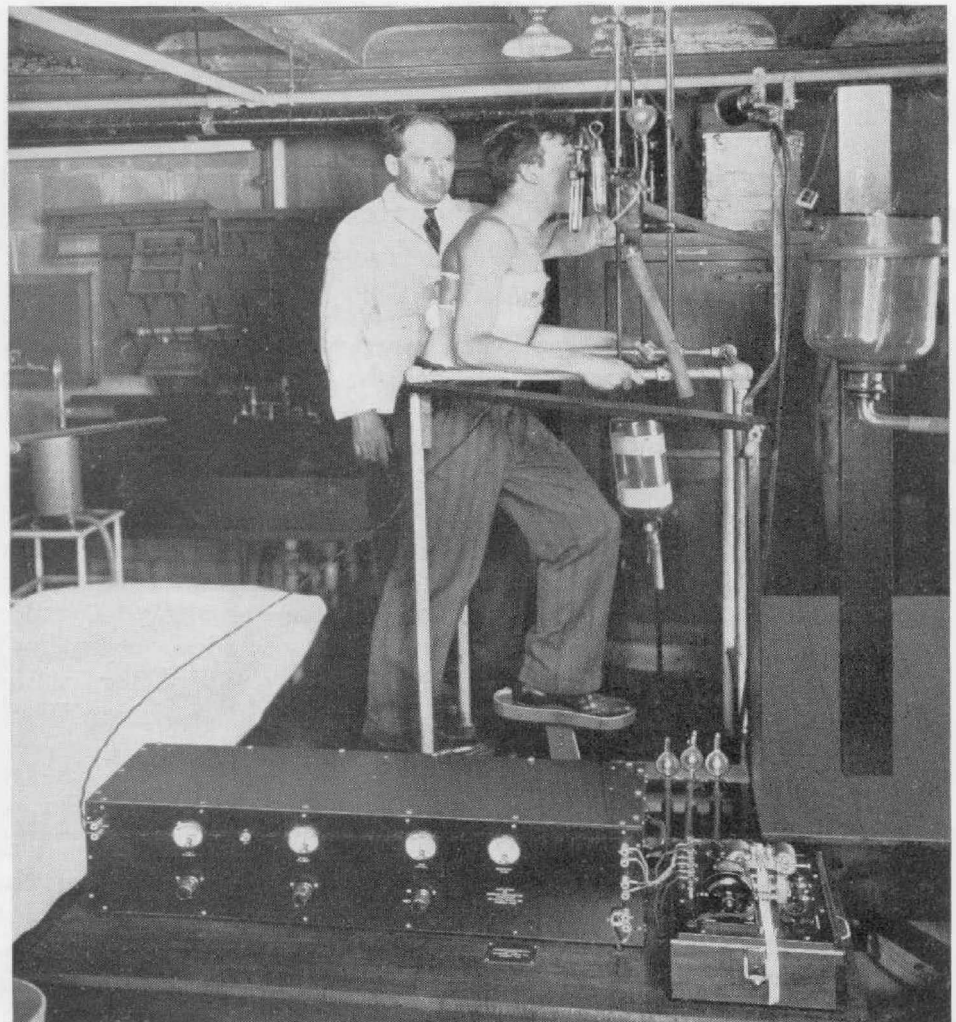
FIGURE 1. The cardiatachometer in use in the laboratory of Dr. A. V. Bock at the Massachusetts General Hospital, Boston. The patient exercises on the treadmill while continuous records of the pulse rate are taken
