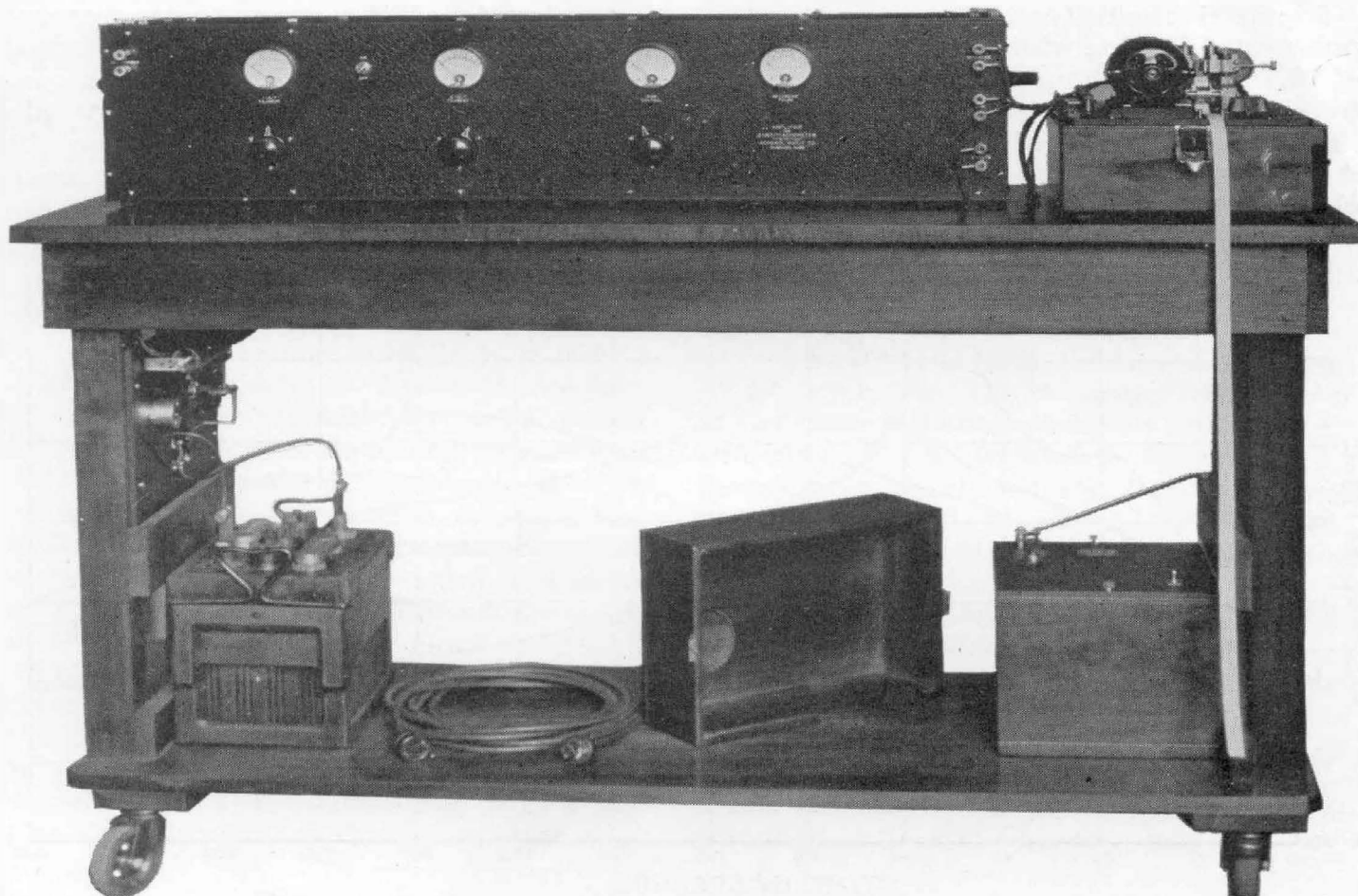
FIGURE 3. The cardi tachometer with amplifiers, syphon recorder, timing device, and power-supply accessories mounted on a casters table
