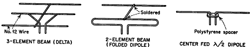
TYPICAL "PLUG-IN" MODEL ANTENNAS FIG. 7
