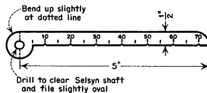
DETAILS OF CURSOR FIG. 6
