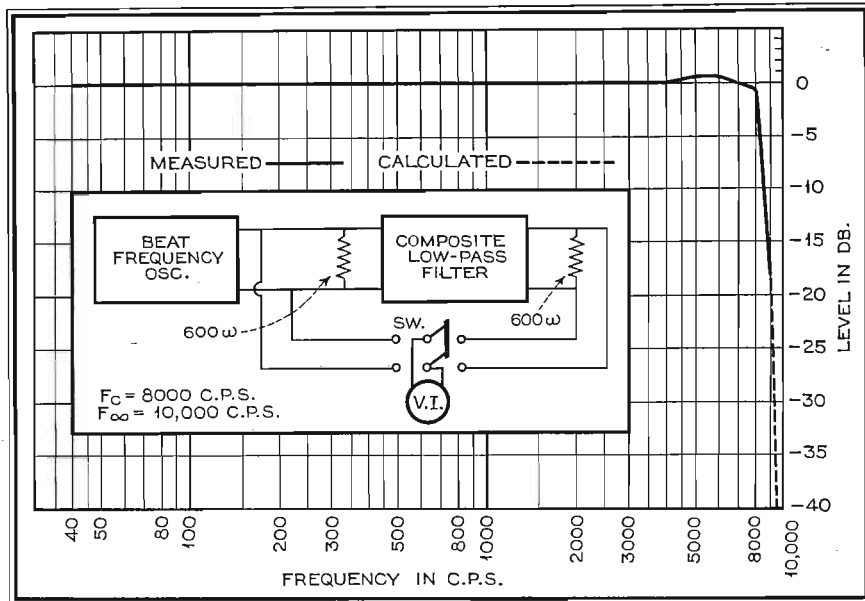
Illustrating the transmission characteristic of the filter.
