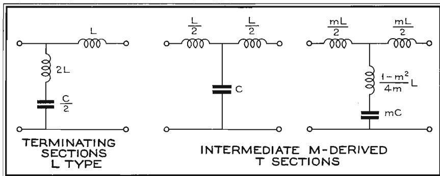
The terminating and intermediate sections.
