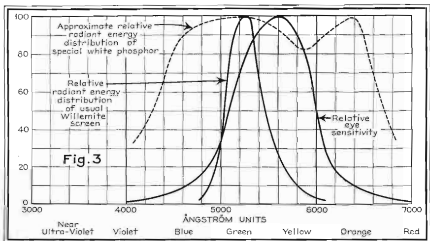
Showing approximate spectral energy distribution compared to eye sensitivity.
