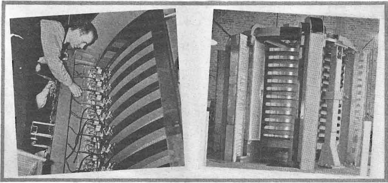
Left: Adjusting one of the 150 optical scanners. Right: A view of the Polyhetor showing mounting method.
