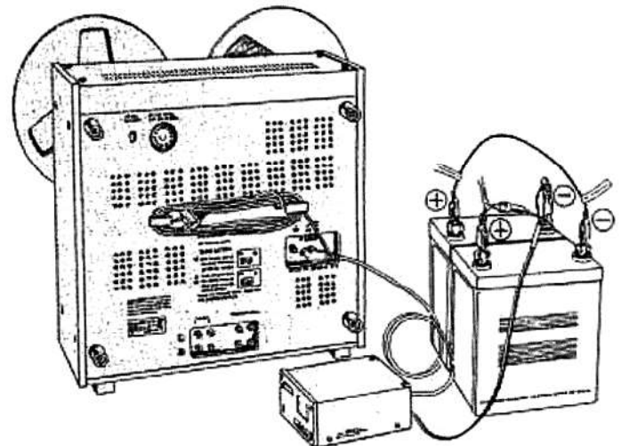
Technics Battery Adaptor (RP-086, optional)
