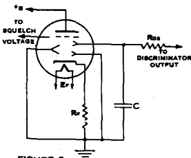
FIGURE 3 SQUELCH VOLTAGE 6 v. (APPROX) OFF CHANNEL
