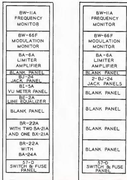
XMTR AT LOCATION REMOTE FROM STUDIO
