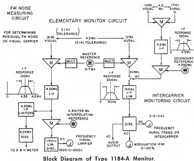
Block Diagram of Type 1184-A Monitor.
