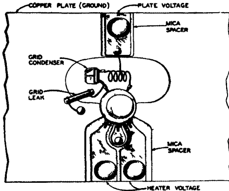
Fig. 11—A typical triode oscillator set-up.
