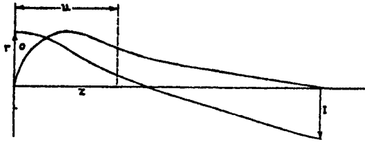
Fig. 5—Electron paths.
