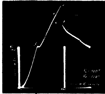
Fig. 19 — Transfer-characteristic oscillogram of special pentode showing the hysteresis and instabilities characteristic of the curve marked \frac{V_a}{V_s} = 0.4 of Figure 11.
