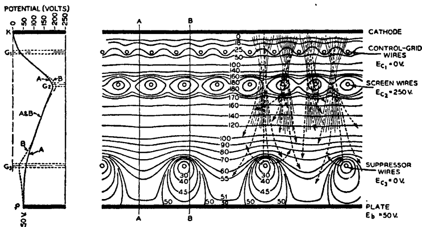
Fig. 12—Plot of potential distribution in a typical power pentode.
