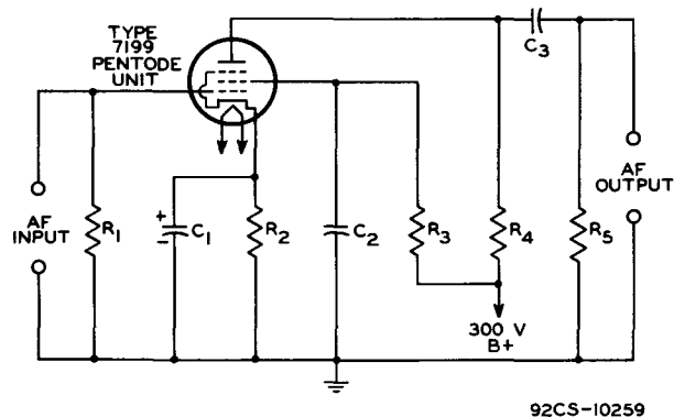
Fig. 6 - General-purpose voltage-amplifier circuit using the pentode unit of an RCA-7199.
