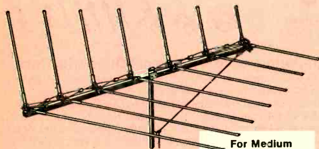
7-Element VHF-FM Medium Area Antenna
