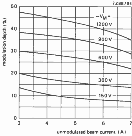
Fig. 7 ABC-operation. Parameter: modulation voltage -V_M (with respect to cathode).
