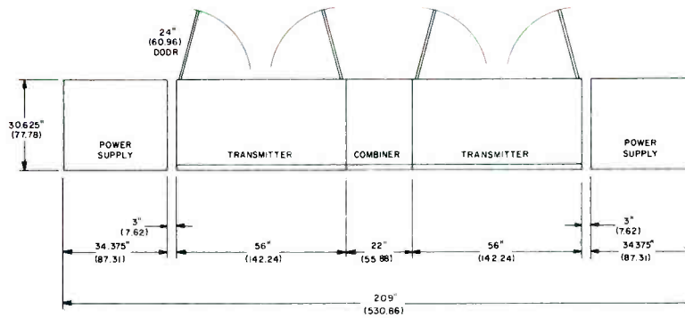
Floor plan
