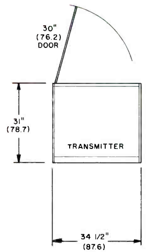
DIMENSIONS IN ( ) GIVEN IN CENTIMETERS
