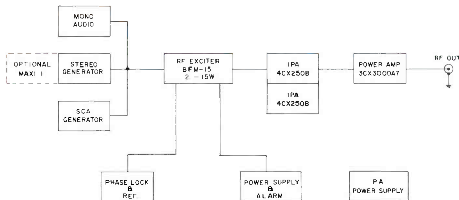
Block diagram
