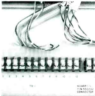
Terminal strip wiring of all inputs
