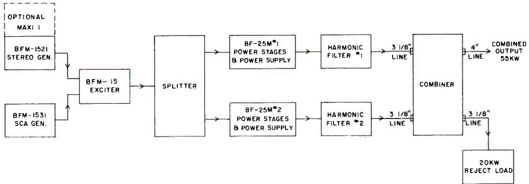
Block diagram
