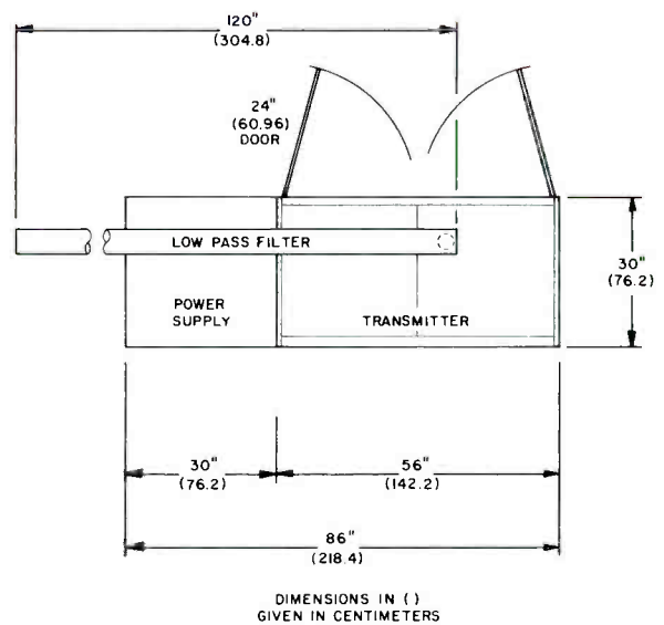
Floor plan
