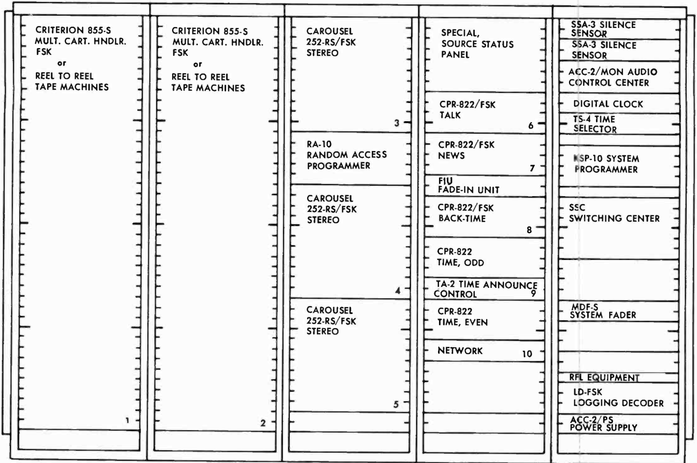
RACK LAYOUT
