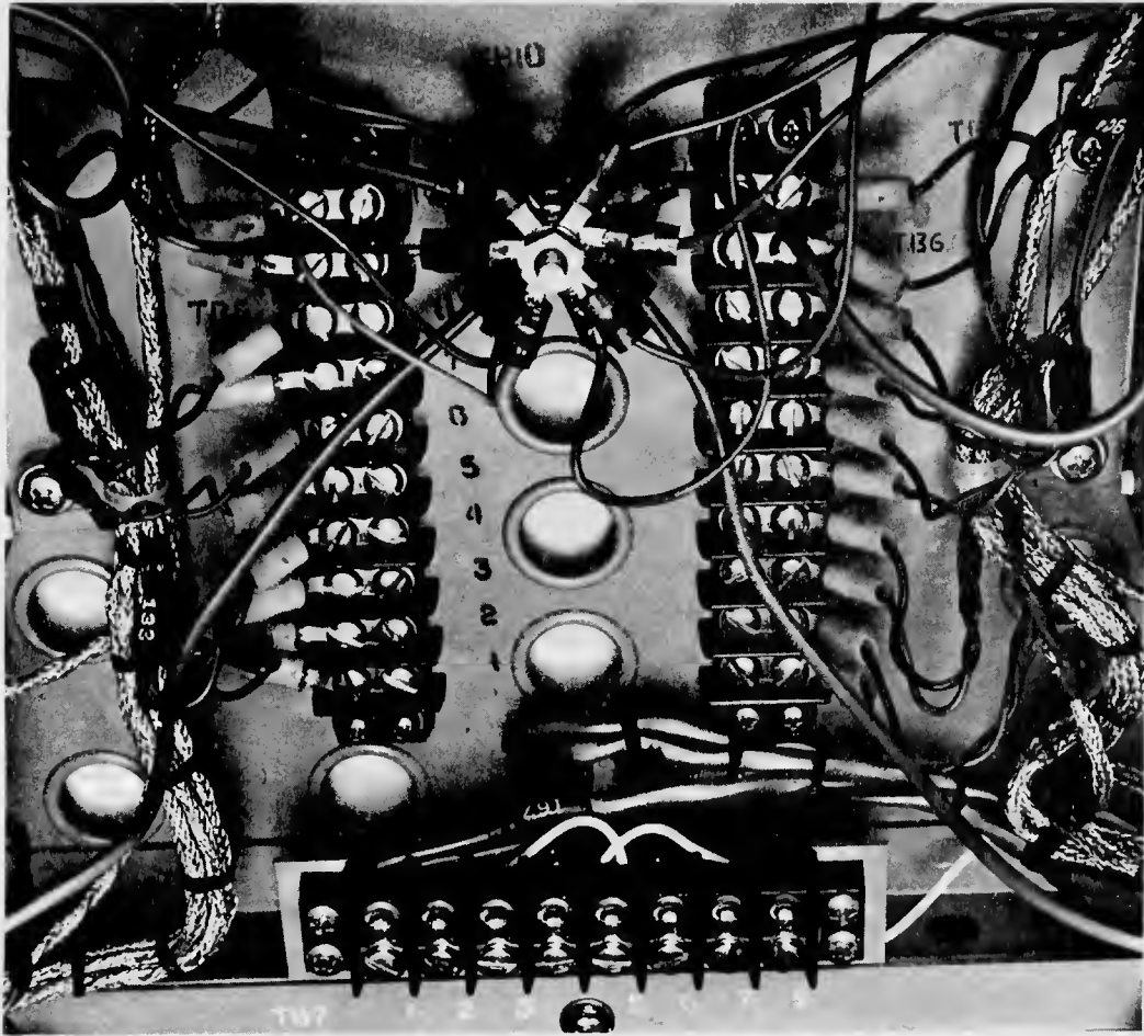
Figure 2-4. Monitor and Intercom Speaker Connections
