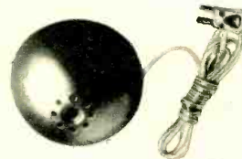
Model OP8002. Lamp base kit for fiber optic displays. Measures 2 1/2" H x 5" dia. Includes bulb, cord, in-line switch. For all IR displays. XM-063J. Wt. 1 lb. .... 4.95
