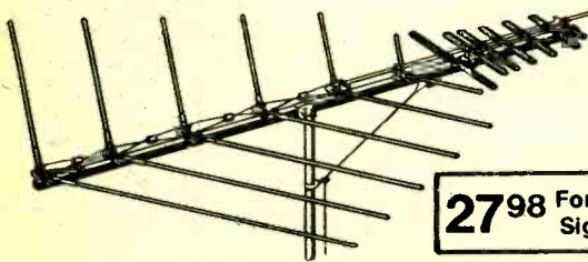
Deluxe 13-Element VHF-UHF-FM Antenna
