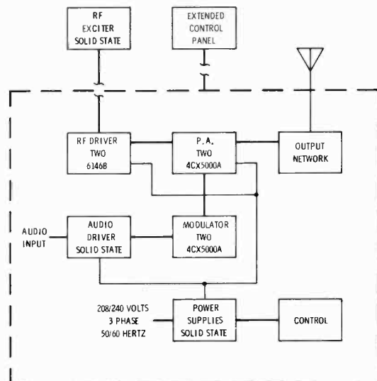
BLOCK DIAGRAM 820F-1
