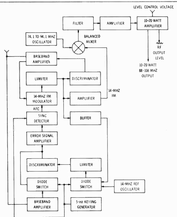
BLOCK DIAGRAM 310Z-1
