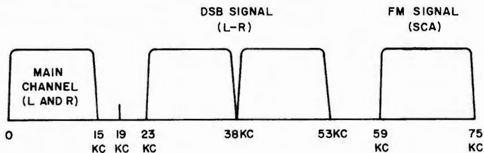
STEREO MULTIPLEX SPECTRUM
