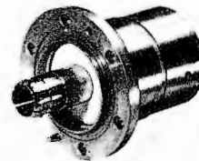
3/4" EIA FLANGE (Male). 50 ohm—TYPE 78R. 75 ohm—TYPE 78R-75. Part No. 099 2314 000-78R
