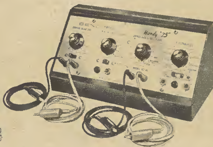
$4995 RC146 Component Substituter $5 monthly
