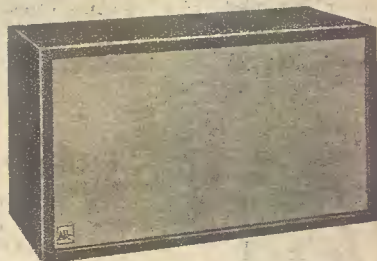
10-in. Woofer, 3½-in. Midrange, 1½-in. Tweeter
