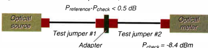
Figure 1b: Insertion loss test procedure; check
