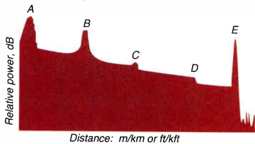
Figure 2: OTDR signature trace
