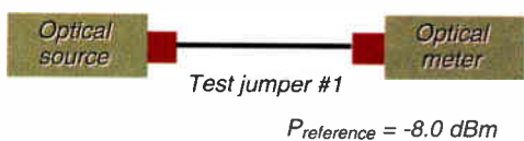
Figure 1a: Insertion loss test procedure; reference
