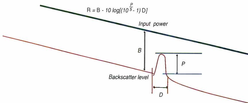
Figure 4: OTDR reflectance measurement
