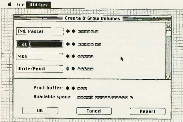
Figure 1: The Create & Grow Volumes Utility of MB Utilities. You can allocate and deallocate space for a volume 400K-byte chunks at a time. These chunks are shown as little floppy disks.
