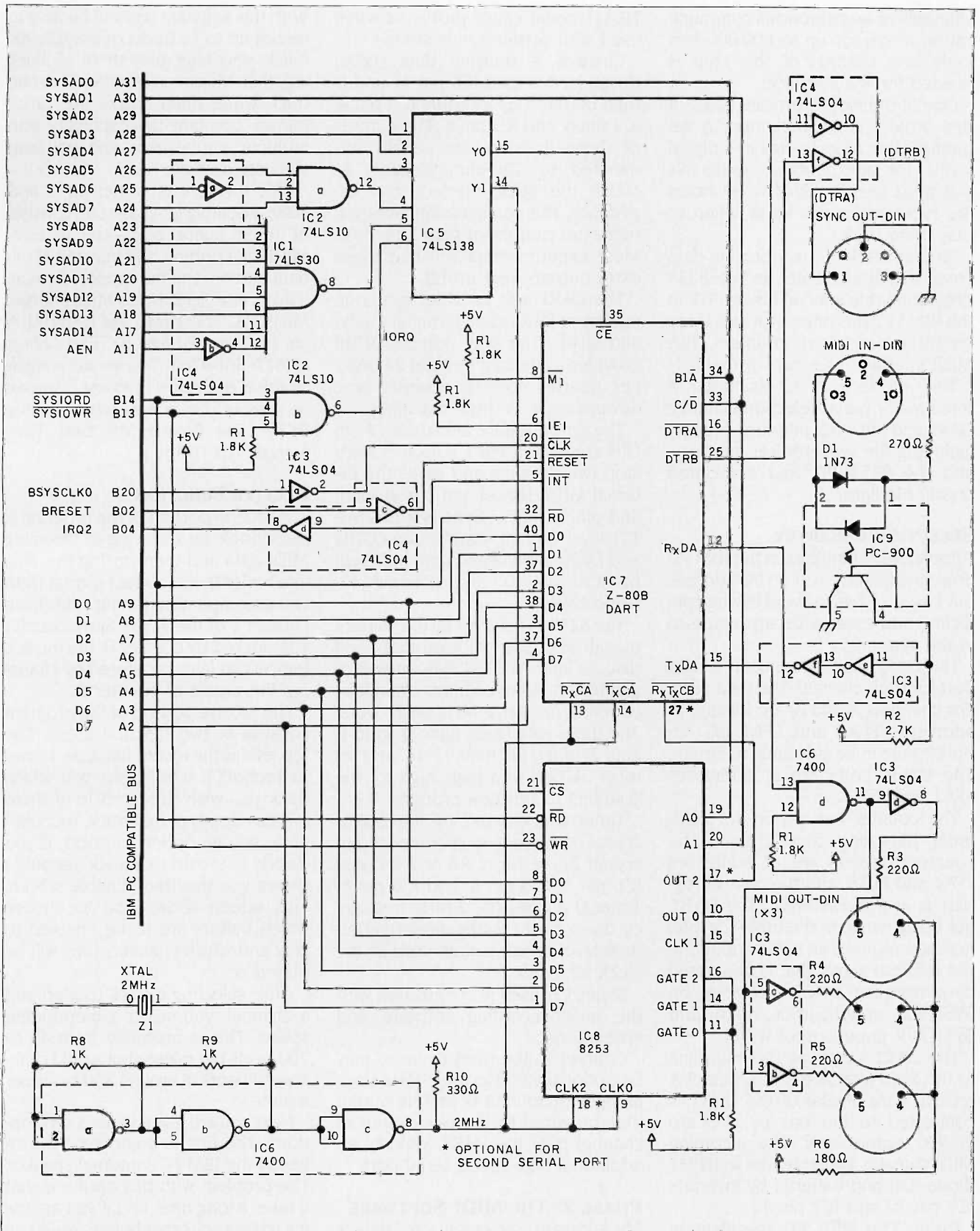
Figure 1: The MIDI 1.0 IBM Board.
