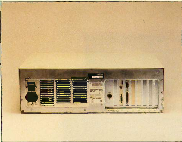
The back panel of the Compaq Deskpro 286. Note the 3-pin DIN power connector for the Compaq monitor.
