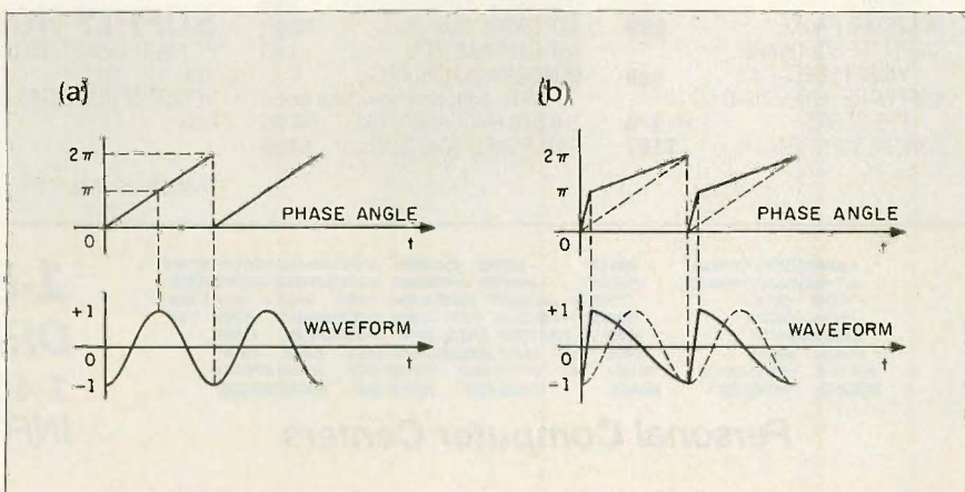
Figure 3: Changing an audio waveform by varying the rate at which a sine lookup table is read out; (a) shows a constant rate of readout, while (b) shows a readout whose rate changes twice per cycle, distorting the sine wave into a sawtooth waveform.
