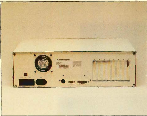
The rear of the Tele-286 showing the power cord receptacle, monitor power cord socket, serial and parallel ports, and access slots for expansion boards with the TeleVideo HRM-100 monitor adapter installed.
