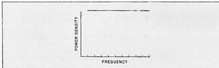
Figure 1a: The power-density spectrum of white, or 1/f^0 , noise.
