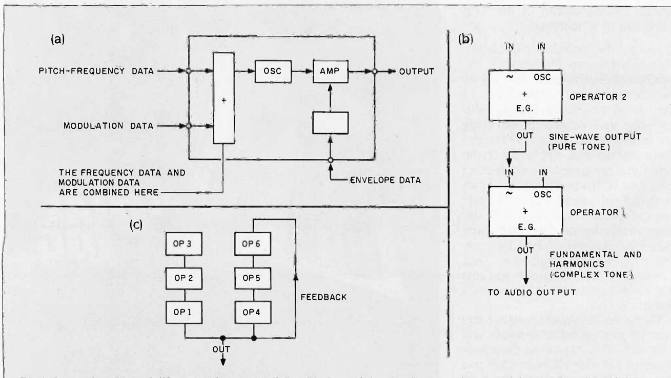
Figure 4: FM waveform-generating building blocks used in Yamaha DX and TX instruments: (a) shows the basic "operator," which you can think of in analog terms as containing a control-summing circuit, oscillator, amplifier, and envelope generator; (b)
