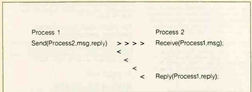
Figure A: The communications interaction between two processes showing the relationship between the Send, Receive, and Reply procedures.
