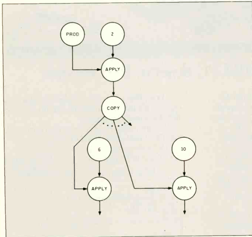
Figure 6: The name produced by the first apply corresponds to a single parameter function that produces the product of all values between 2 and the parameter value.
