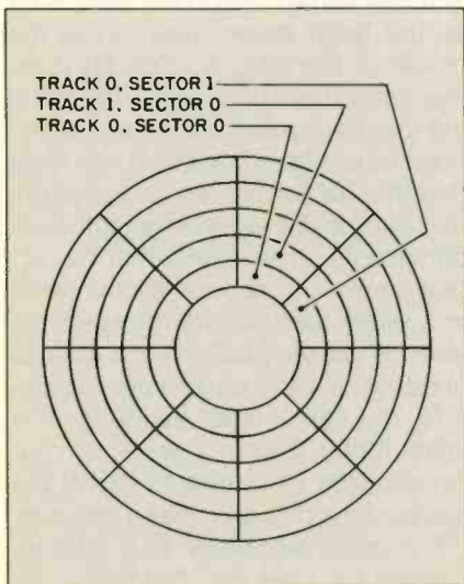
Figure 1: The sector organization of a typical CAV (constant angular velocity) magnetic disk. The sectors on the outer tracks are physically longer than those on the inner tracks and are organized in concentric rings.
