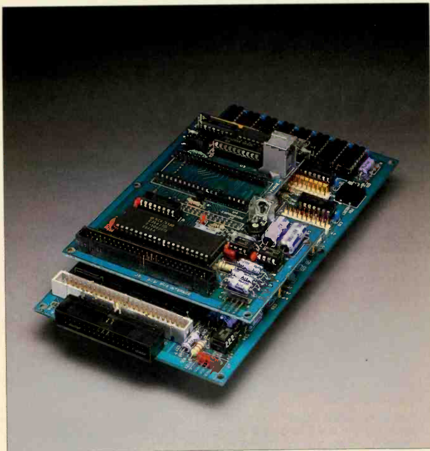
Photo 2: The COMM180 SCSI interface board rides piggyback on the SB180 single-board computer. The NCR 5380 is the large chip toward the front. Note the empty socket for the MOSART modem chip (see the November 1985 Circuit Cellar for a description of the MOSART).
