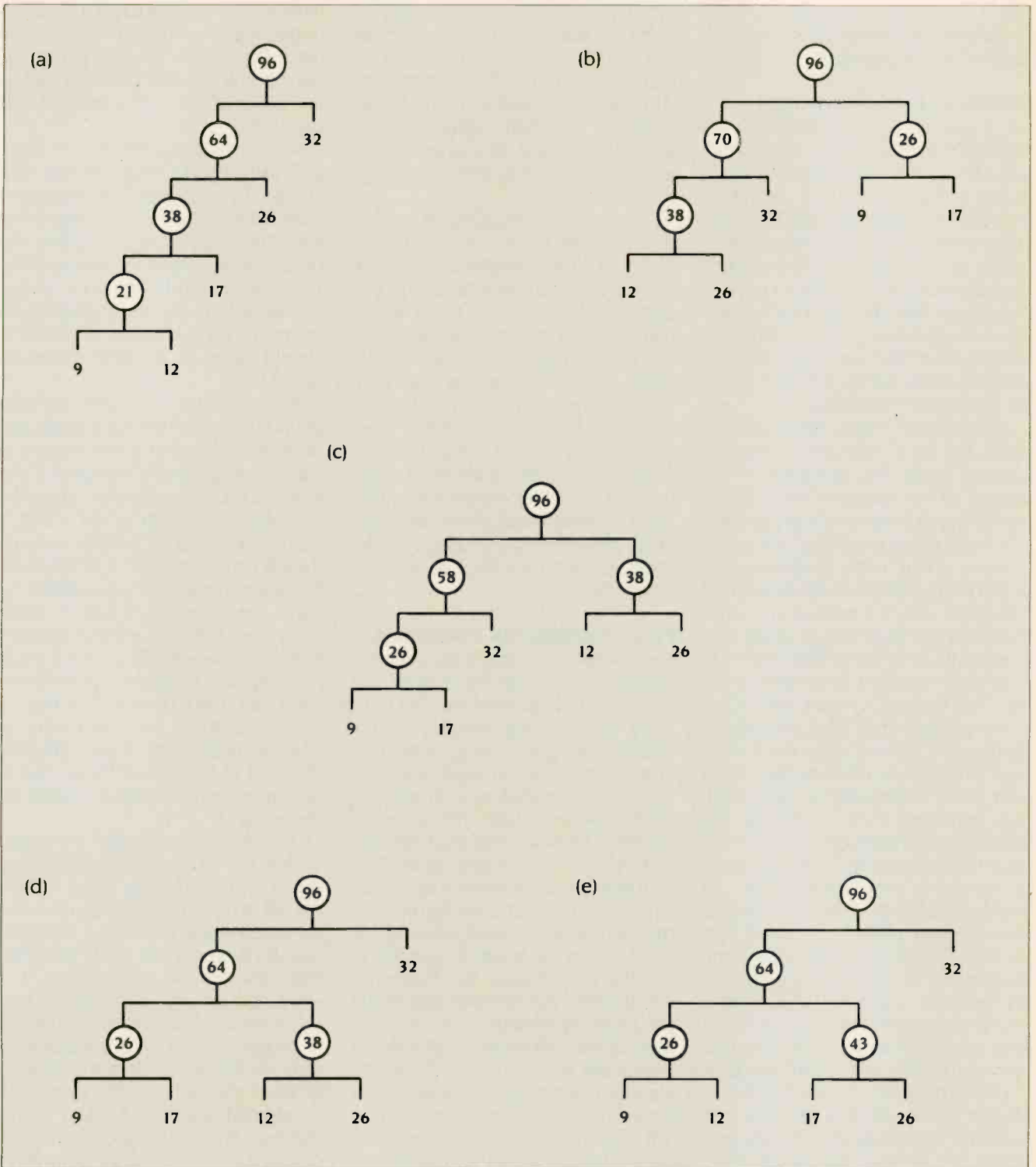
Figure 5: Given the subtrees 9, 12, 17, 26, and 32, examine some trees that diverge from the tree produced by the Huffman algorithm. For now, look at only the frequencies of these subtrees and ignore the characters these frequencies correspond to: (a) The tree the Huffman algorithm would build from these subtrees; (b) The subtree with the second-lowest frequency (12) is lower in the tree than the subtree with the lowest frequency; (c) The subtree with the second-lowest frequency is higher in the tree than the subtree with the lowest frequency; (d) The second-lowest frequency is at the same level as the lowest frequency; (e) Swapping 12 and 17 gives a tree that diverges from the tree that would be produced by the Huffman algorithm at a later point than that of figure 5d and yet still has the same weighted path length of the tree of figure 5d.
