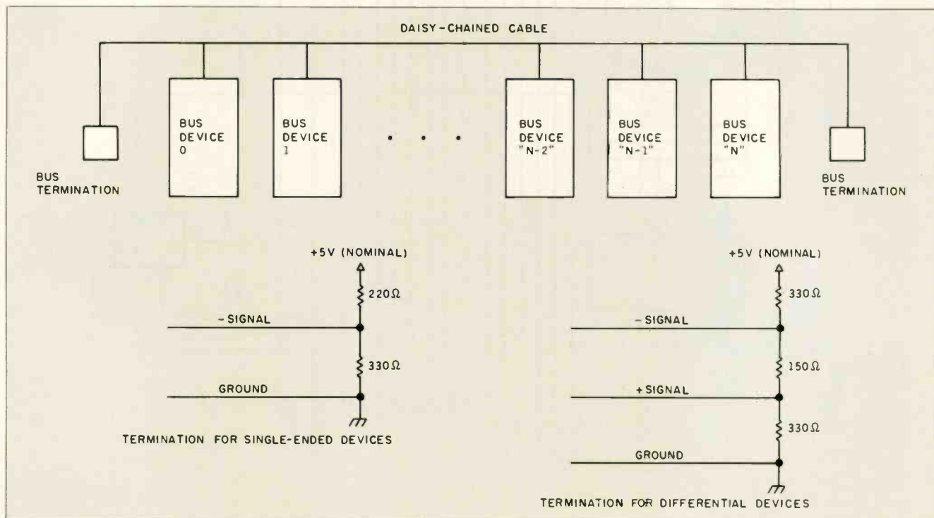
Figure 7: SCSI bus termination hardware characteristics.
