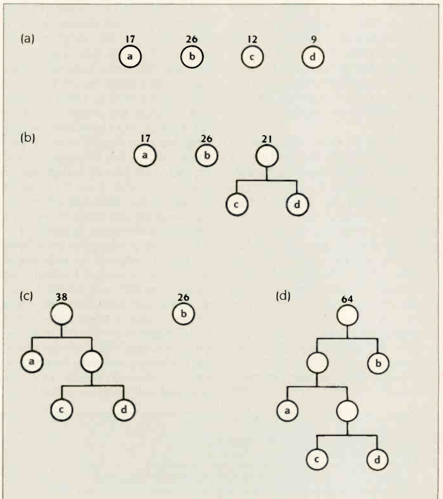
Figure 2: How the Huffman algorithm constructs the tree in figure 1: (a) It begins with a list of characters and their frequencies; (b) It combines the characters with the lowest frequencies, "c" and "d," into a subtree and puts the subtree in the list; (c) Now the character "a" and the newly constructed subtree have the lowest frequencies, so they are combined; (d) Finally, the remaining character is combined with the subtree to form the completed code tree.
