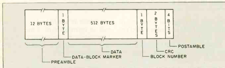
Figure 6: A typical data-block format used for tape backup systems, the QIC-24 format.
