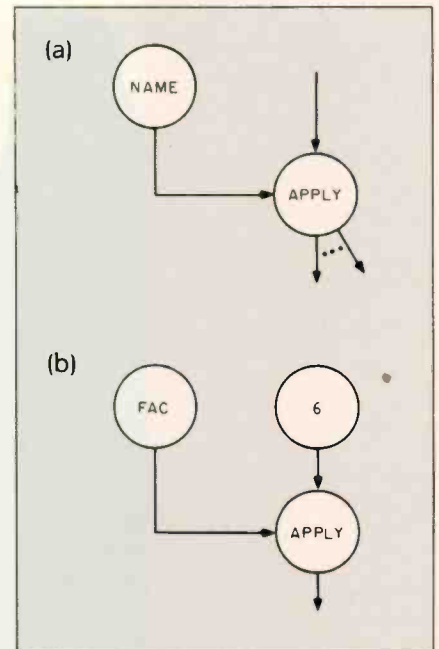
Figure 4: The apply node takes two inputs, a function name or closure and a parameter value. Function names can be written explicitly at the node or passed on an input arc as are function closures. As its result, the apply node produces a value or a function closure depending on whether the applied function was a first-order function or a higher-order function.
