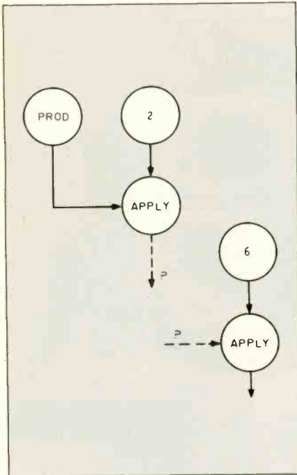
Figure 5: What value does the first apply node produce? What function is supplied to the second?
