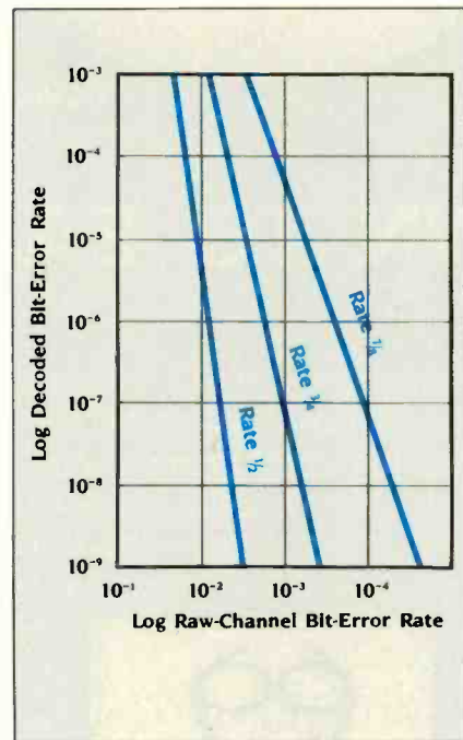
Figure 2: The performance of three RS codes against random occurrence of bit errors. All three use code words consisting of 32 five-bit bytes. The rate 1/2 code has 16 information bytes and 16 redundancy bytes per block, an RS(32,16) code. The rate 3/4 code is RS(32,24), and the rate 7/8 code is RS(32,28).
