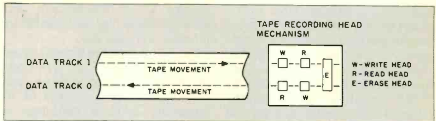
Figure 2: The integral part of a tape-drive unit, the recording head, consists of read, write, and erase heads. This diagram shows two tracks of a multiple-track tape system. Note the placement of the read heads after the write heads, for the purpose of error detection.
