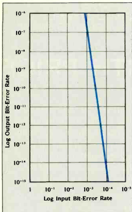
Figure 1: The relationship between the raw error rate and the corrected error rate using an RS(220,204) code. Code words consist of 220 eight-bit bytes, of which 204 bytes are information and 16 bytes are redundancy, for a code rate of 92.73 percent. The figure assumes random, independent bit errors. Performance against somewhat "bursty" errors is even better.
