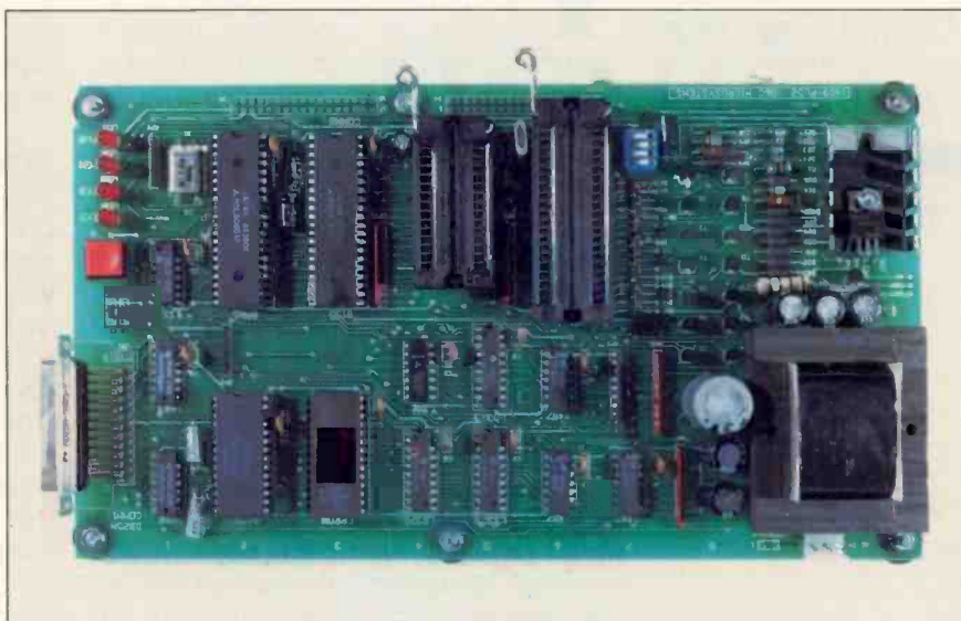
Photo 1: Assembled and tested (bare-board version) 1409-13A EPROM Programmer.
