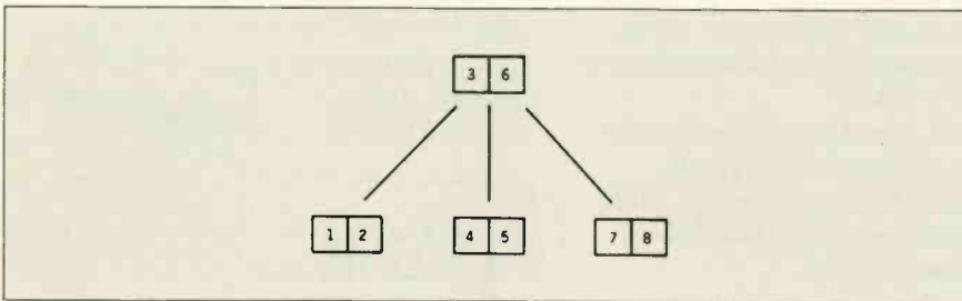
Figure 3a: A two-level B-tree with a block size of 2.
