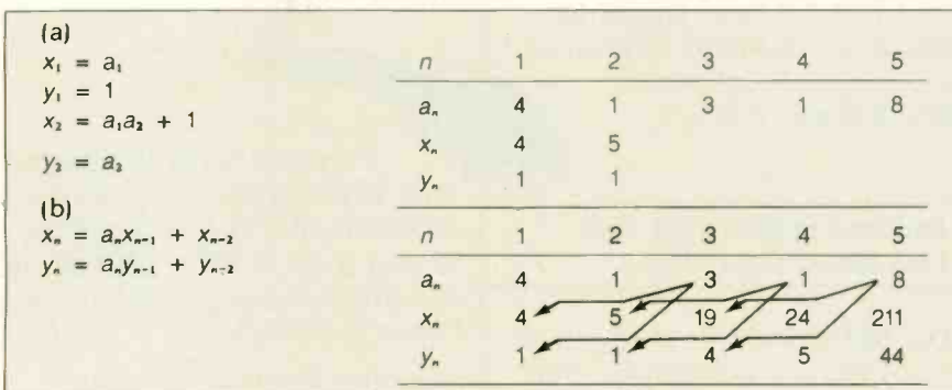
Figure 4: (a) The first two x and y values; (b) the flow diagram for subsequent x and y values.
