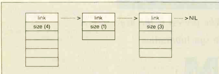
Figure 1: A chain of memory blocks. Each block begins with a MemoryDescriptor record that points to the next block.
