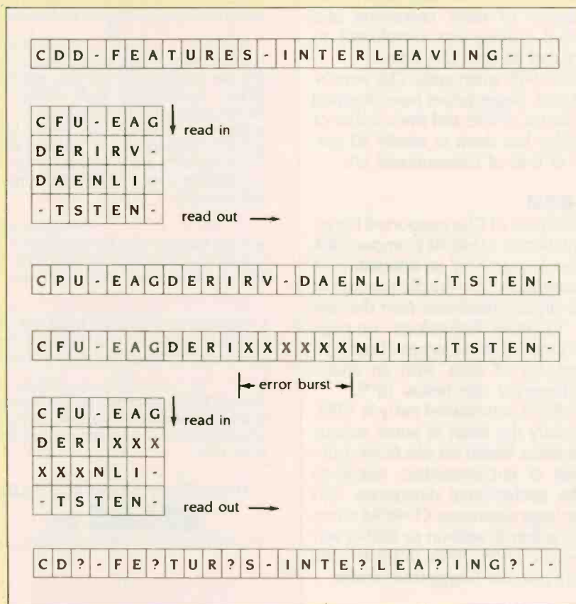
Figure A: In this example of data interleaving, the long error burst (XXXXXX) is separated into shorter ones that can be handled by the error-correction decoder.
