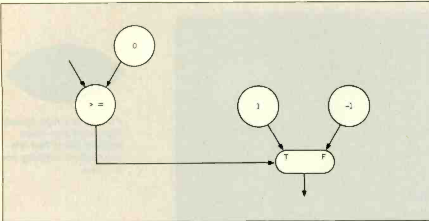
Figure 7: This is a program that returns the sign of its input, which arrives in the "left" input field of instruction 2. As we noted earlier, outputs emanate from a particular instruction but are not directed toward any instruction. This is represented in the code by an asterisk in the output list of an instruction.
