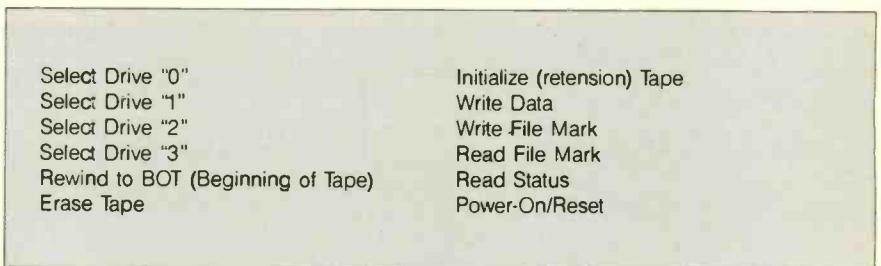
Figure 3: These QIC-02 commands are typical of commands that a tape-drive controller uses to send information to and from a backup tape.
