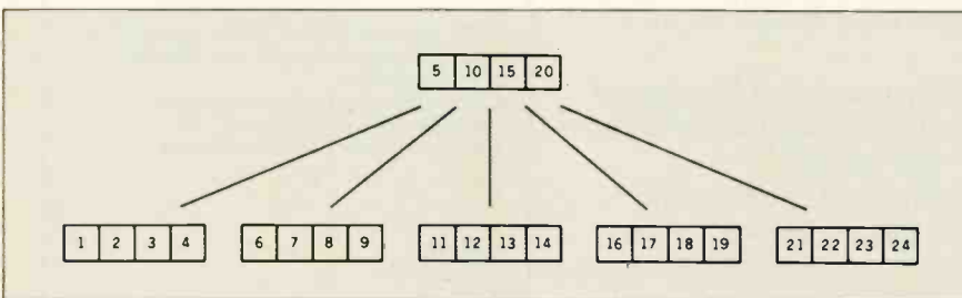
Figure 3b: A two-level B-tree with a block size of 4. Note that doubling the block size from figure 3a more than doubles the number of records the tree can hold.
