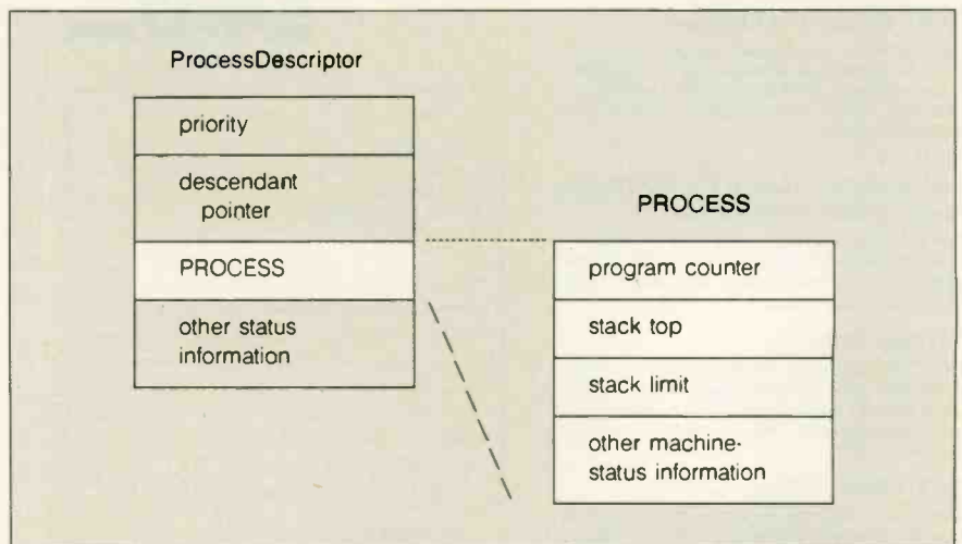
Figure 3: A ProcessDescriptor including the machine-dependent PROCESS variable provided by Modula-2.
