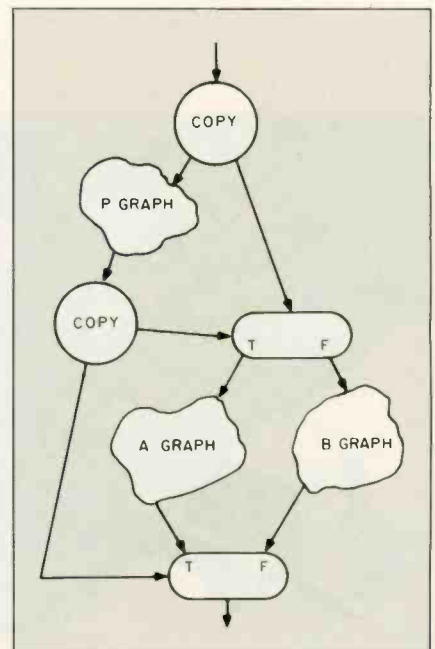
Figure 2: A possible graph for the defining expression of the Hope function: dec f : num -> num; --- f(a) <= if P then A else B; where P, A, and B are arbitrary expressions referring only to a.
