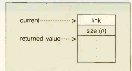
Figure 2: The returned value is a pointer equal to the current pointer value plus the size of the MemoryDescriptor record.
