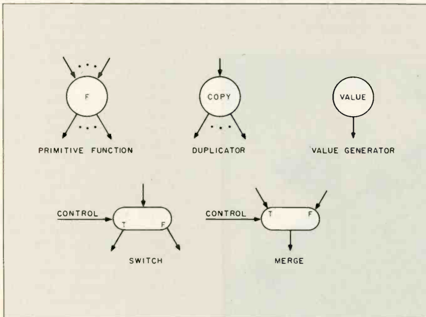
Figure 1: In these diagrams of the basic operators, the data flow is directed down the page. Inputs to and outputs from a graph are shown as arcs that are connected to the graph only at one end.
