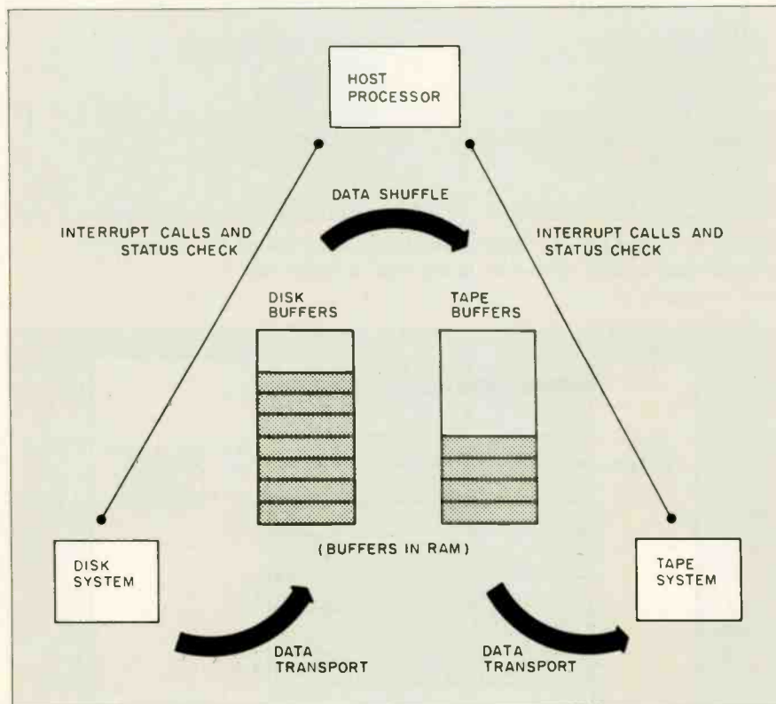
Figure 5: In the process of data exchange from the host computer system to the tape backup drive, the tape software uses the host system's RAM as a buffer to manipulate data blocks.
