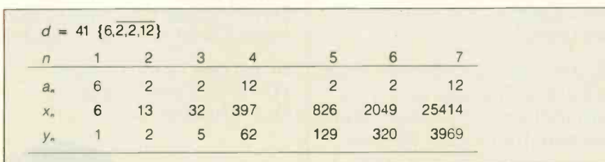
Figure 5: The completed chart of x, y values for x^2 - 41y^2 = 1 .
