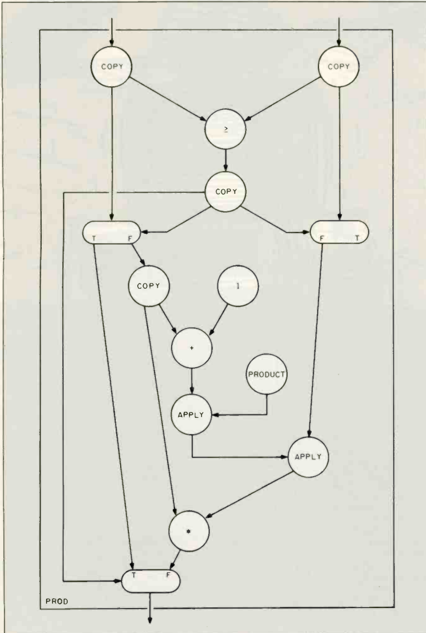
Figure 3: The box defines the graph as a function. Note that the T output from the right switch is omitted because the value of b is not required when the condition is satisfied. Any application of prod will require two apply nodes.
