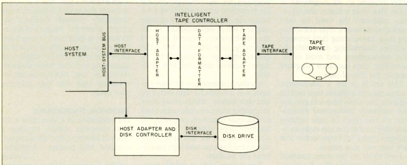
Figure 1: A tape backup system typically consists of an intelligent tape controller with interfaces to the host computer system and the tape drive itself. Depending on the system, all or part of this controller may be incorporated into the host system (as an add-on card) or into the tape-drive unit.
