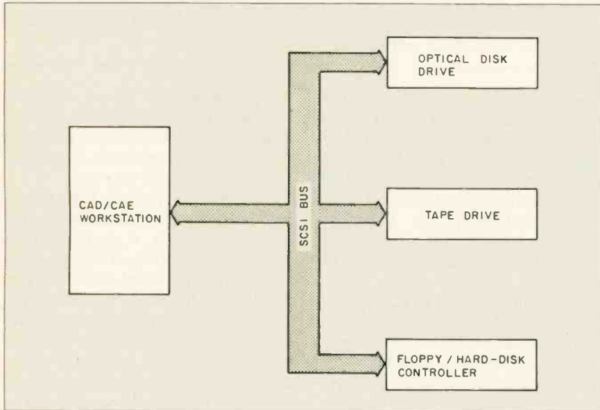
Figure 3: A single-user/multitasking SCSI system.
