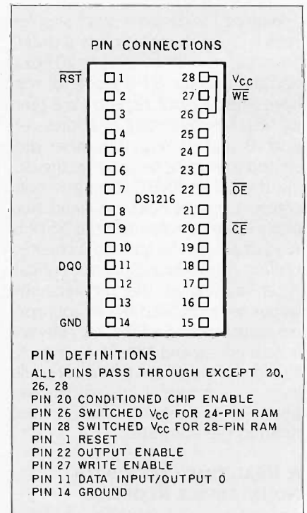
Figure 7: A pin-out for the DS1216 SmartWatch.
