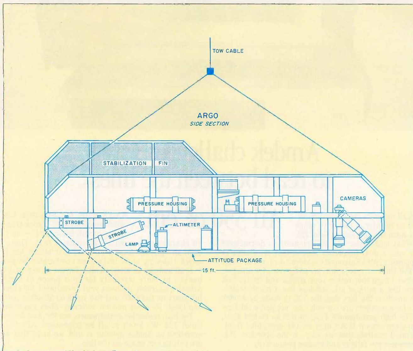
Figure 2: This drawing of the Argo shows the tow cable, pressure housings, cameras, and lights. Other housings hold the altimeter, attitude package (depth, heading, heave, etc.), and control and communication electronics.
