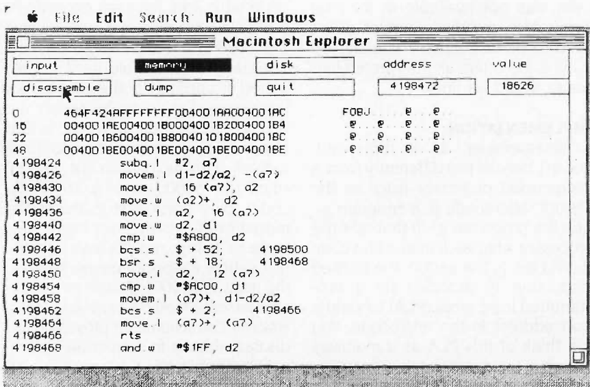
Figure 2: Shown is the screen of the Macintosh Explorer. Note that the memory path is in reverse video, indicating that it is active. You can see a dump of the beginning of memory and a disassembly starting at address 4198424.
