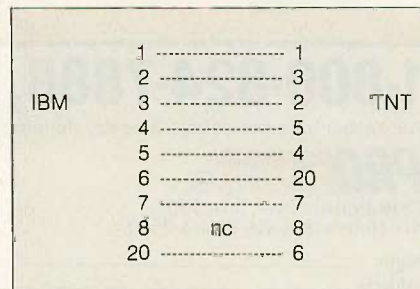
Figure 1: The diagram for construction of a null-modem cable.
