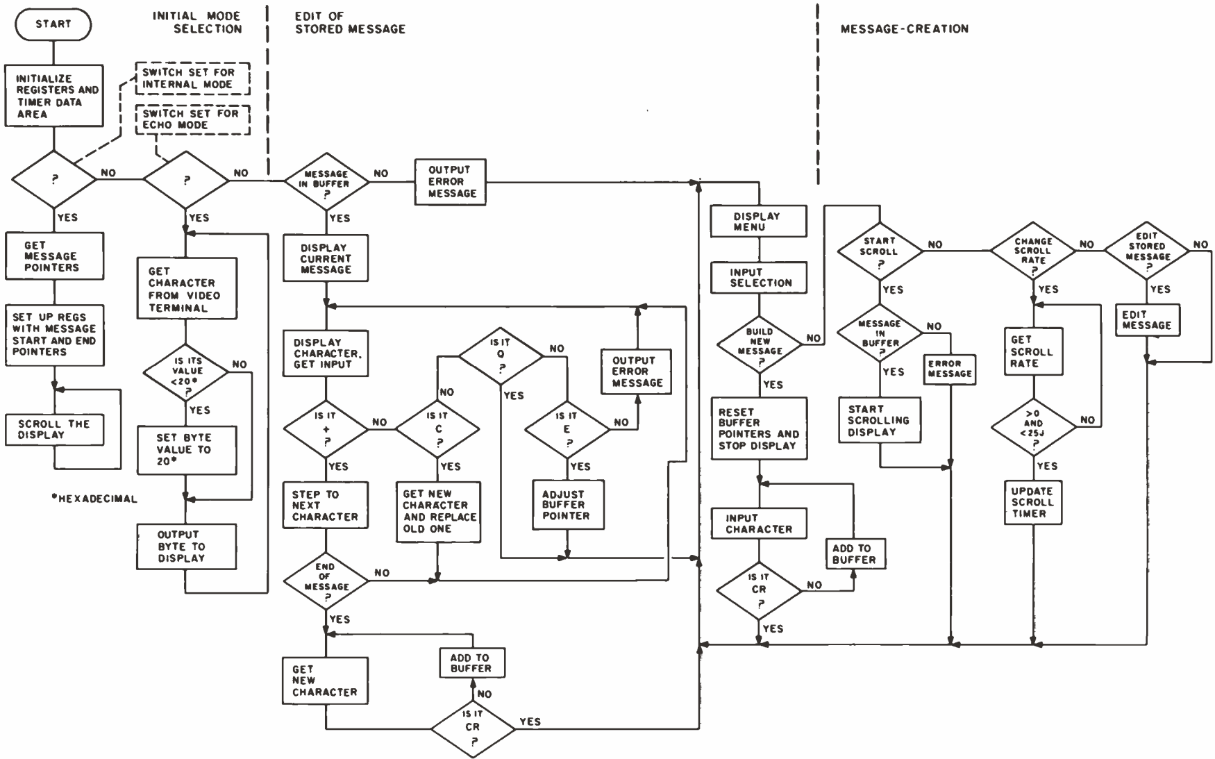
Figure 7: Flowchart of the display-controller software for the Z8-BASIC System Controller. Some modes of operation are selected by DIP-switch settings on the Z8 board.
