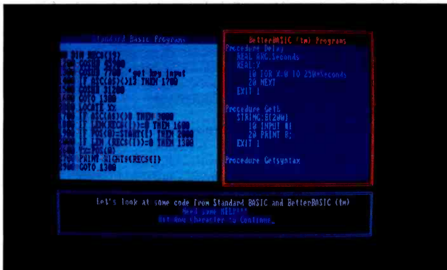
Photo 3: Windows, with standard BASIC on the left and BetterBASIC source code on the right.
