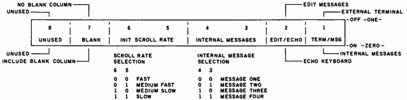
Figure 9: Options that can be selected by DIP-switch settings on the Z8 board. When used without a terminal, the controller can be thereby set up to start automatically and display one of four prestored messages at one of four scrolling rates.
