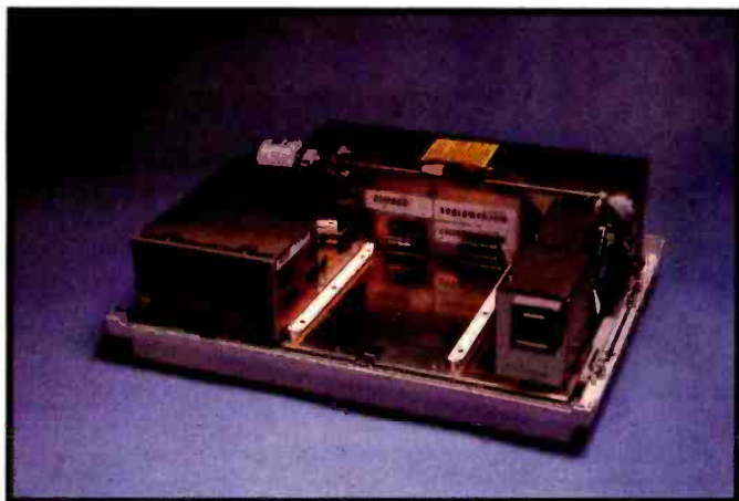
Photo 4: A look under the Rainbow's cover. The power supply is along the rear edge. The RX50 drive is on the right. The empty spot in the middle will accept another RX50 drive or a 5¼-inch 10-megabyte hard-disk drive.
