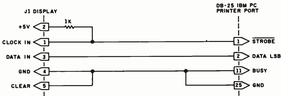
Figure 4: The parallel printer port on an IBM PC's Monochrome Display Adapter can be wired to drive the LED display using only the least significant data bit.
