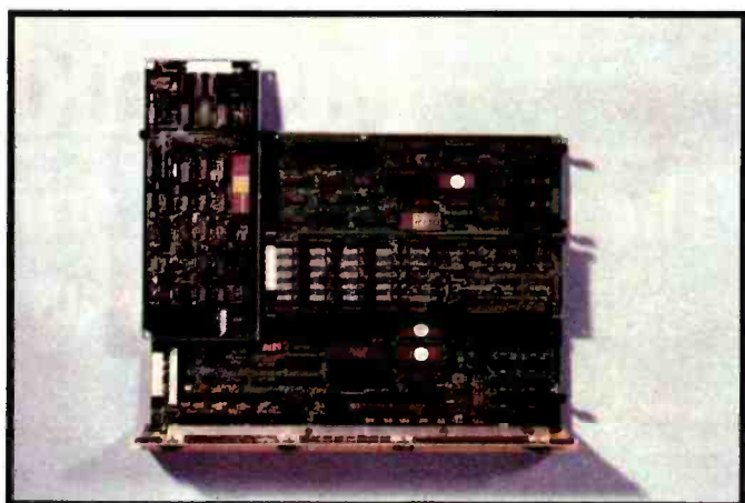
Photo 5: The Rainbow's motherboard. The rear of the board is on the bottom. The disk controller is the vertical board on the left. The 3- by 10-inch board that runs horizontally across the middle is the optional RAM expansion board.
