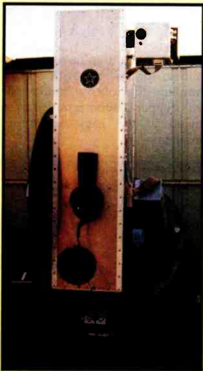
Photo 1: The original Automatic Photoelectric Telescope (APT) at the Fairborn Observatory West in Phoenix, Arizona. The photometer that "looks" at the stars is the box attached to the top right of the telescope. The large-diameter disk on the left side of the telescope moves the telescope in declination while the large disk at the bottom rear moves the telescope in right ascension. This telescope finds, centers, and measures stars automatically.
