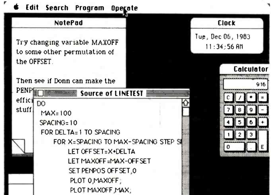
Figure 3: Macintosh desk accessories run concurrently with program development. The Note Pad (in the background) has eight pages and holds 256 bytes per page.
