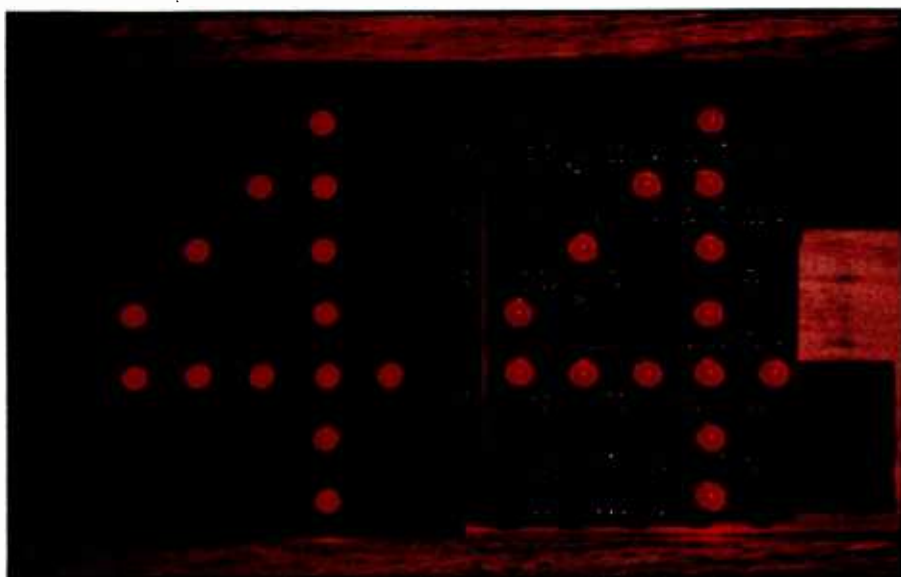
Photo 4: These examples of the numeral "4" were produced by the same bit pattern used in listing 1, but under the control of the Z8-BASIC System Controller. The red plastic filter over the left segment greatly improves the appearance of the display.
