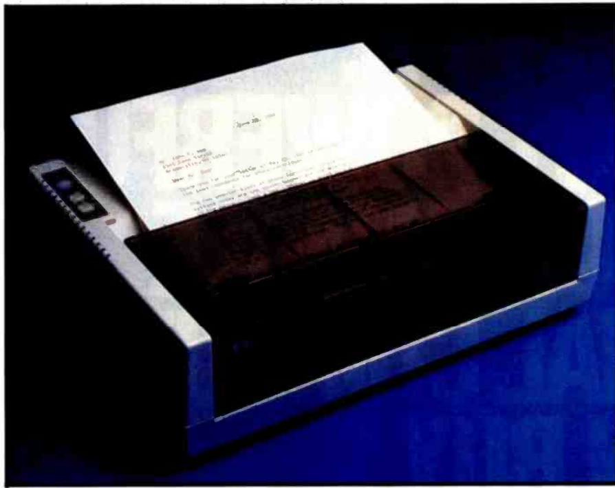
Photo 4: The Hewlett-Packard 2225 ink-jet printer. HP engineers claim a noise level below 50 decibels—quieter than normal conversation.
