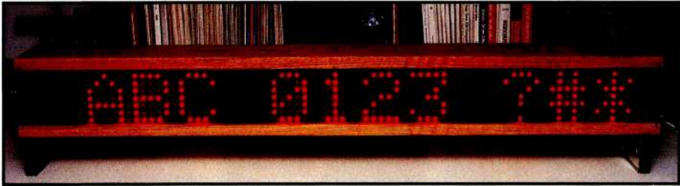
Photo 6: In the finished project, multiple character segments are linked and housed together in an attractive wooden enclosure. Either canned or live messages can be written or continuously scrolled across the array under control of the Z8 software.
