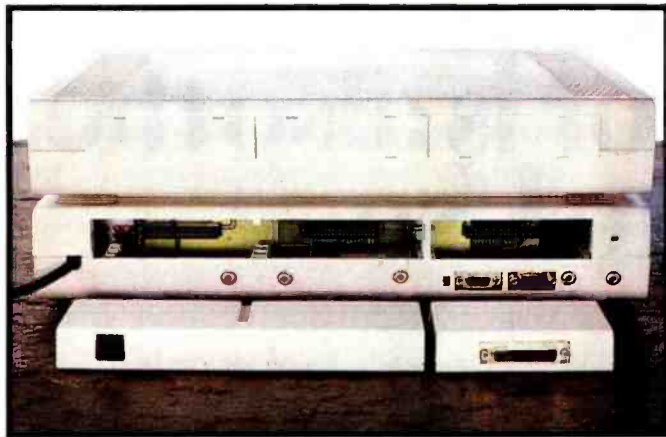
Photo 7: Photo 7a shows the rear panels of the System Unit (bottom) and Expansion Unit (top). Each unit contains connections for three I/O modules. At the bottom left of photo 7a is a modem module (which takes two module slots). The connectors on the bottom rear of the System Unit are, from left to right, audio out, composite video out, RF-modulated video out, channel 3/channel 4 switch, RGB video out, external sync in, auxiliary serial in, and auxiliary serial out. At the bottom right of photo 7a is the RS-232C module; photo 7b shows the same module disassembled.
