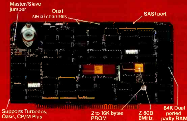
SBC 300 single board computer
