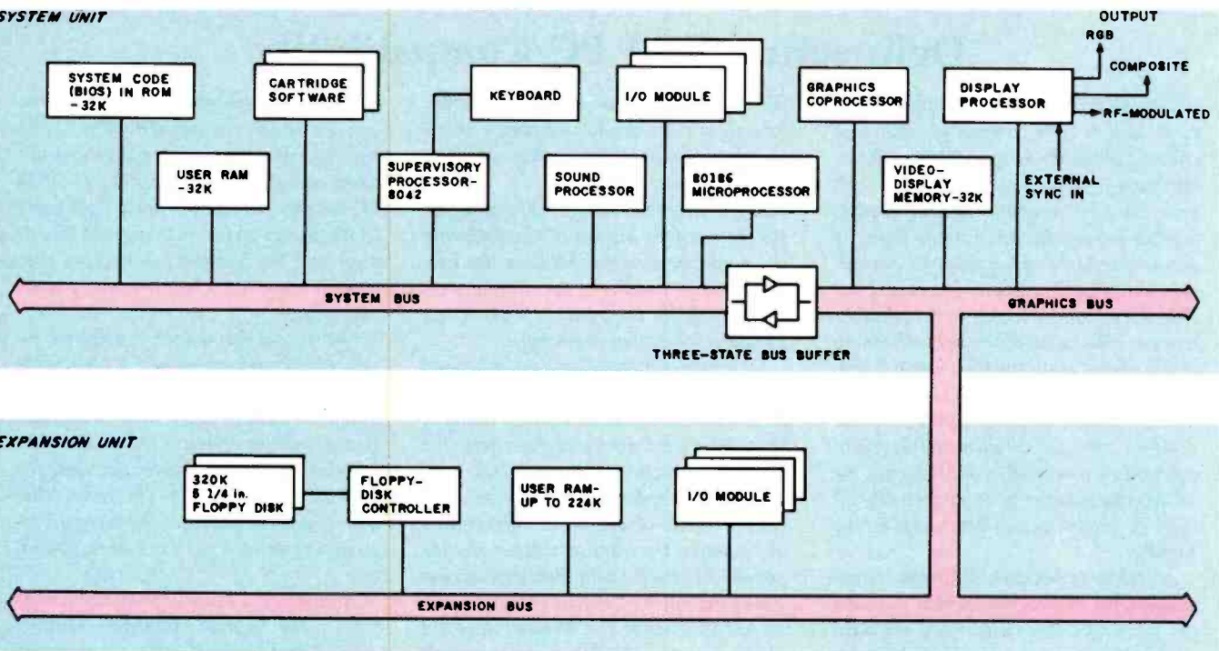
Figure 1: Block diagram of the Mindset personal computer.
