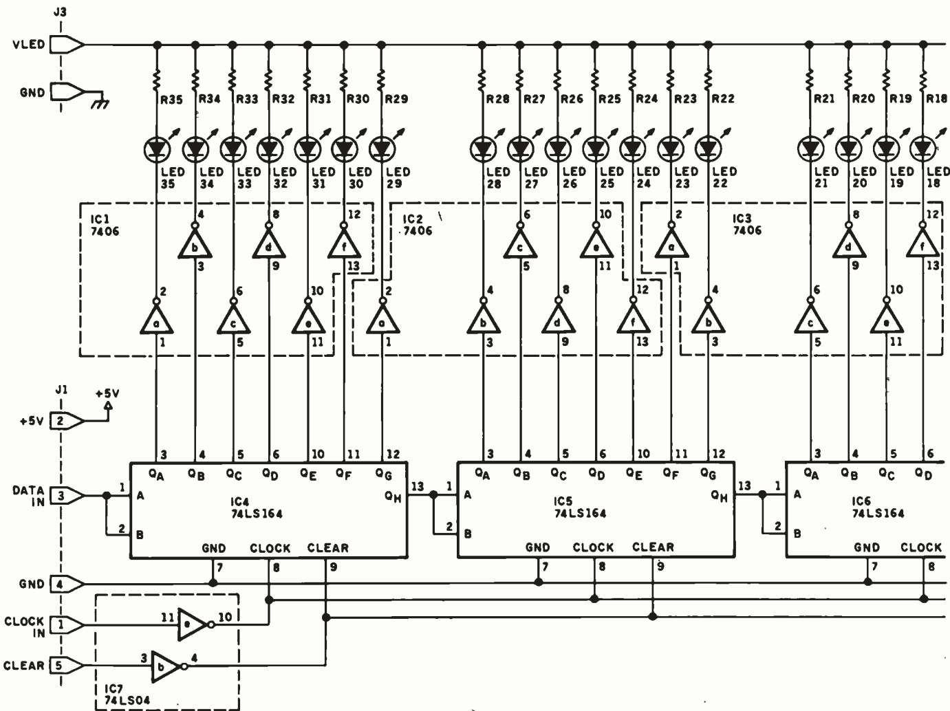
Figure 1: Schematic diagram of one of the character-segment subassemblies for the scrolling LED display.
