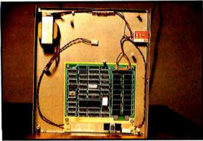
Photo 2: The Co-Power-88 main processor board, mounted on the ATR8000's bottom tray.
