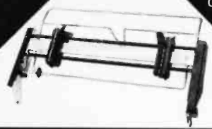
RS 700 Mechanical Sheet Feeder. Automatic feeder with mechanical control mechanism. No electronics required. Driven forward by printer platen.
