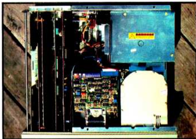
Photo 2: Inside the system unit (the front is at the bottom) you can see part of the system unit board that contains the 8088 microprocessor, 64K bytes of RAM, a disk controller, a parallel printer port, and expansion slots. The memory-expansion board is located on the left side of the unit toward the front. From left to right: the expansion cards installed in this unit are the synchronous/asynchronous communications card, the CRT controller card with the video graphics card mounted piggyback on it, the 300/1200-bps auto-dial/auto-answer modem, and the Winchester controller card. The disk drives obscure a large portion of the system board. The power supply is located at the right rear corner of the unit.
