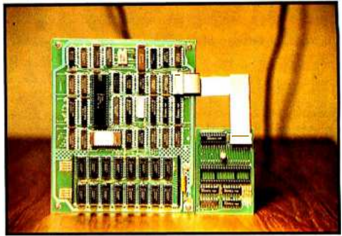
Photo 3: The Co-Power-88 main processor board and Z80 adapter board.
