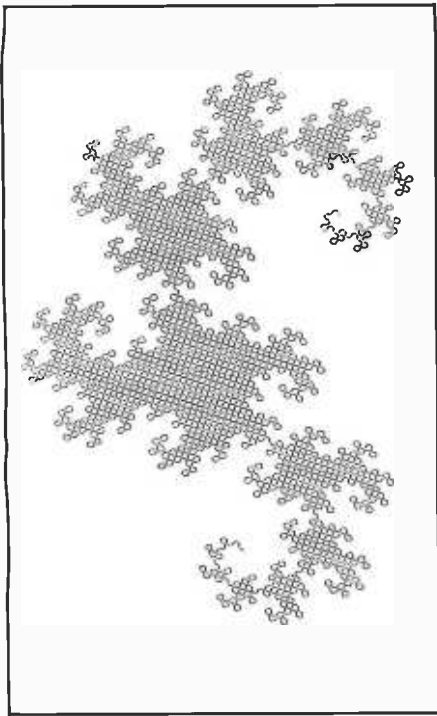
Figure 1: An order-12 classical dragon curve. This dragon curve was constructed on a TRS-80 Model I using the Gendrag program. It was printed on an IDS Paper Tiger, used with the Diskplot print routines as a plotting device.
