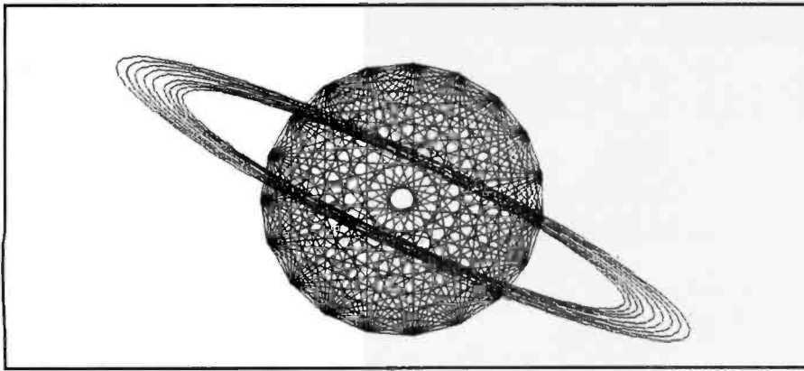
Figure 12: A 19-vertex n-gon overlaid by concentric ellipses. Drawn with Diskplot.
